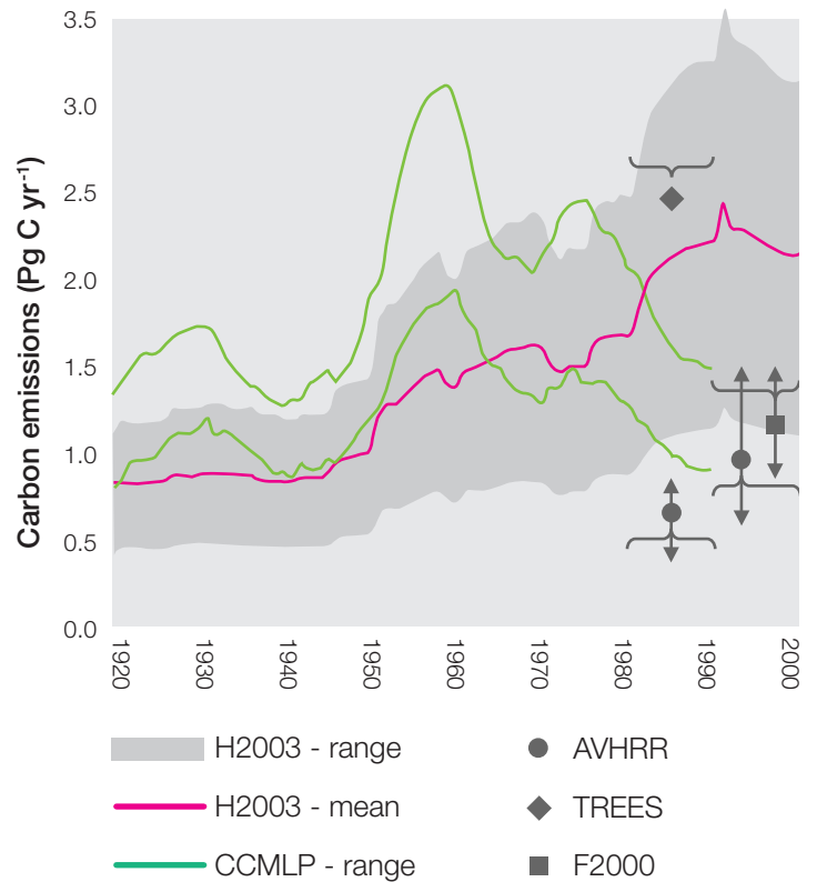
Figure 6. Intercomparison of five different estimates of carbon emissions from global land-cover change.
