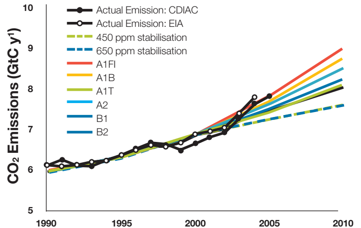
Figure 4: Actual global CO 2 emissions as compared to IPCC scenarios
