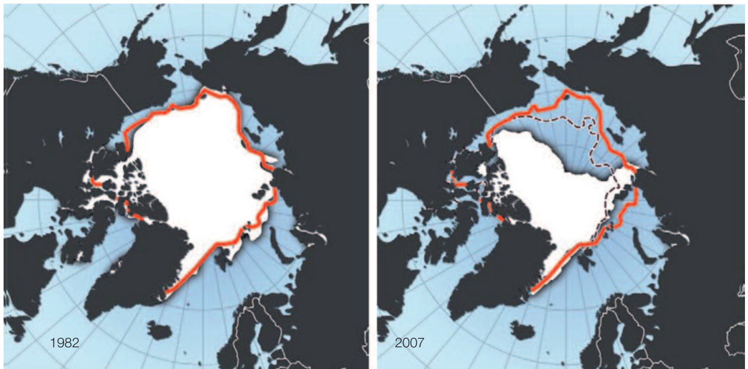
Figure 2: Arctic Sea-Ice Trends
