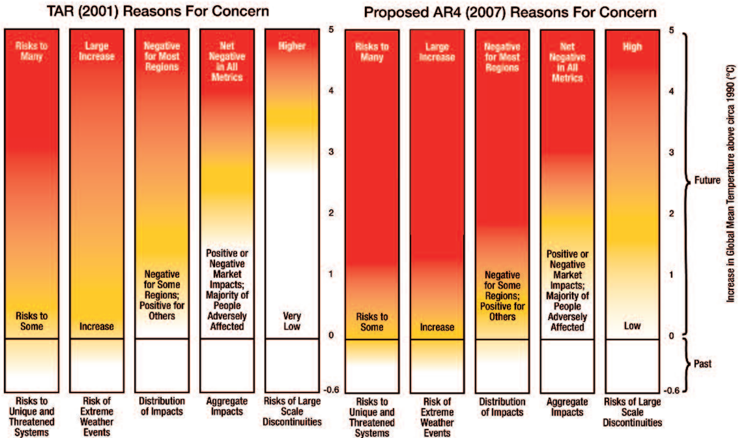
Figure 3: Reasons for Concern: The increasing danger to the planet from rising temperatures.
