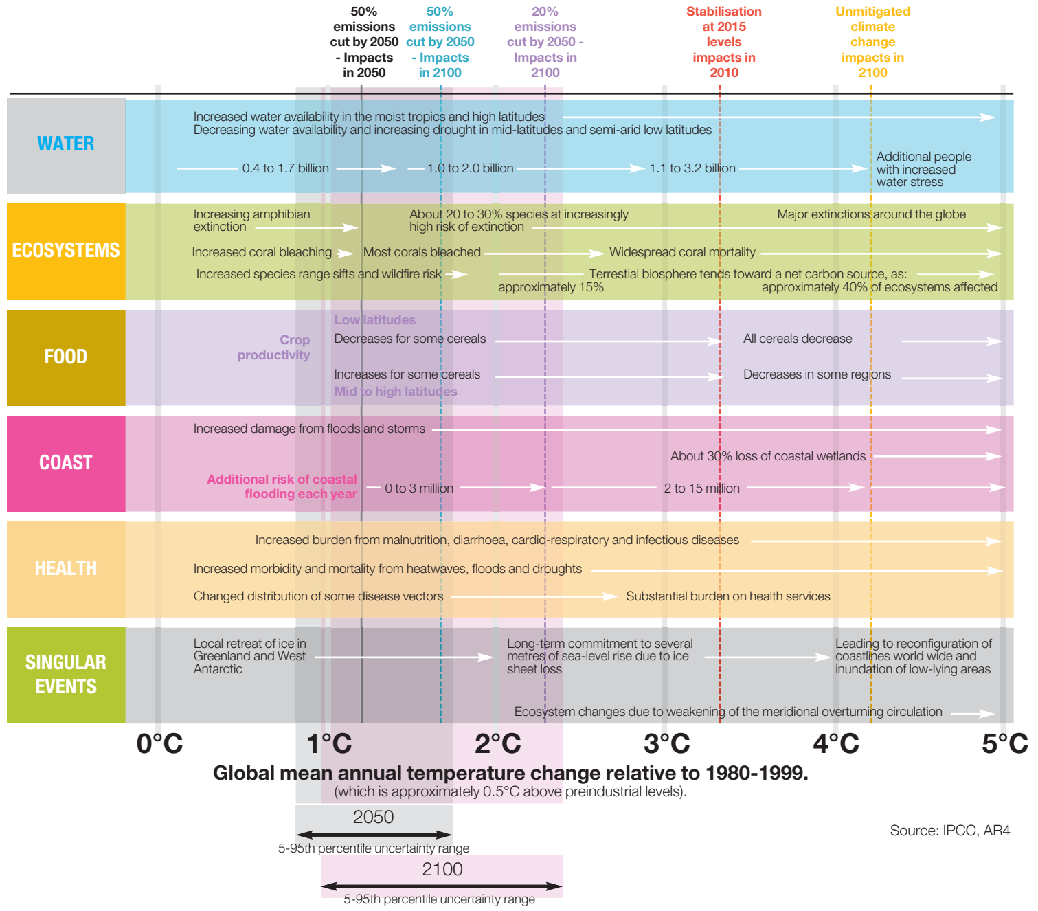
Figure 1: Examples of impacts associated with global average temperature change
