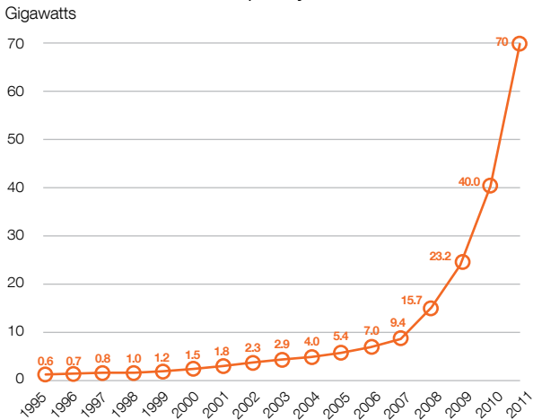
Solar PV: total world capacity 1995-2011
