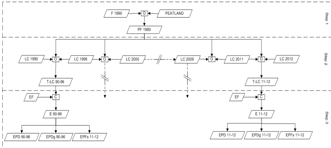
Figure 3. Flow chart of Calculation flow chart of peat decomposition emission calculation from peat decomposition in deforested peat forests from forested peat 1990. “LC” is land cover, “EF” is Emission Factor for peat decomposition, “E”, “T-LC” is transition area matrix, “EPD” is Emission Peat from Deforestation, “EPDg” is Emission Peat from Forest Degradation, “EPFs” is Emission Peat from Secondary Forest, “O” is Overlay, “C” is Calculate. “LC Annual” is the annual rate of deforestation within one interval (e.g. 1990 – 1996) the proportion of annual deforestation derived from annual loss of primary forest data (Margono et al., 2014), “Dp” is deforested areas and degraded forest occurred in peat forests. Revisi is required
