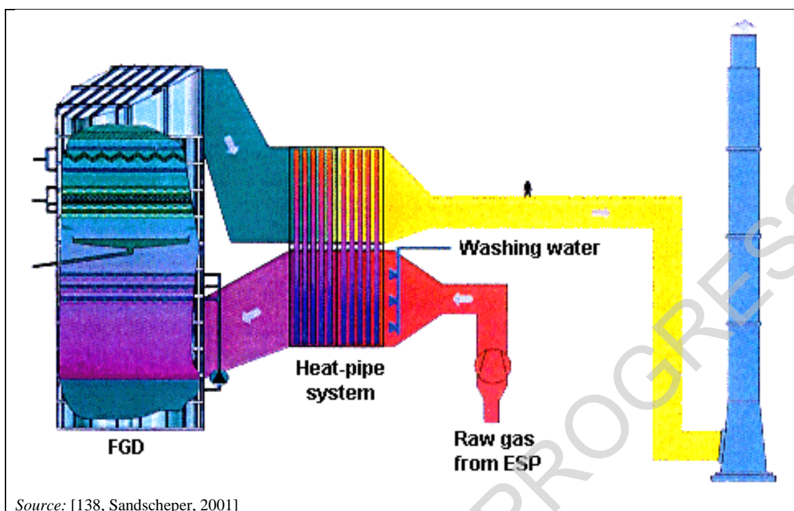
Figure 5.36: Heat displacement around the FGD unit
