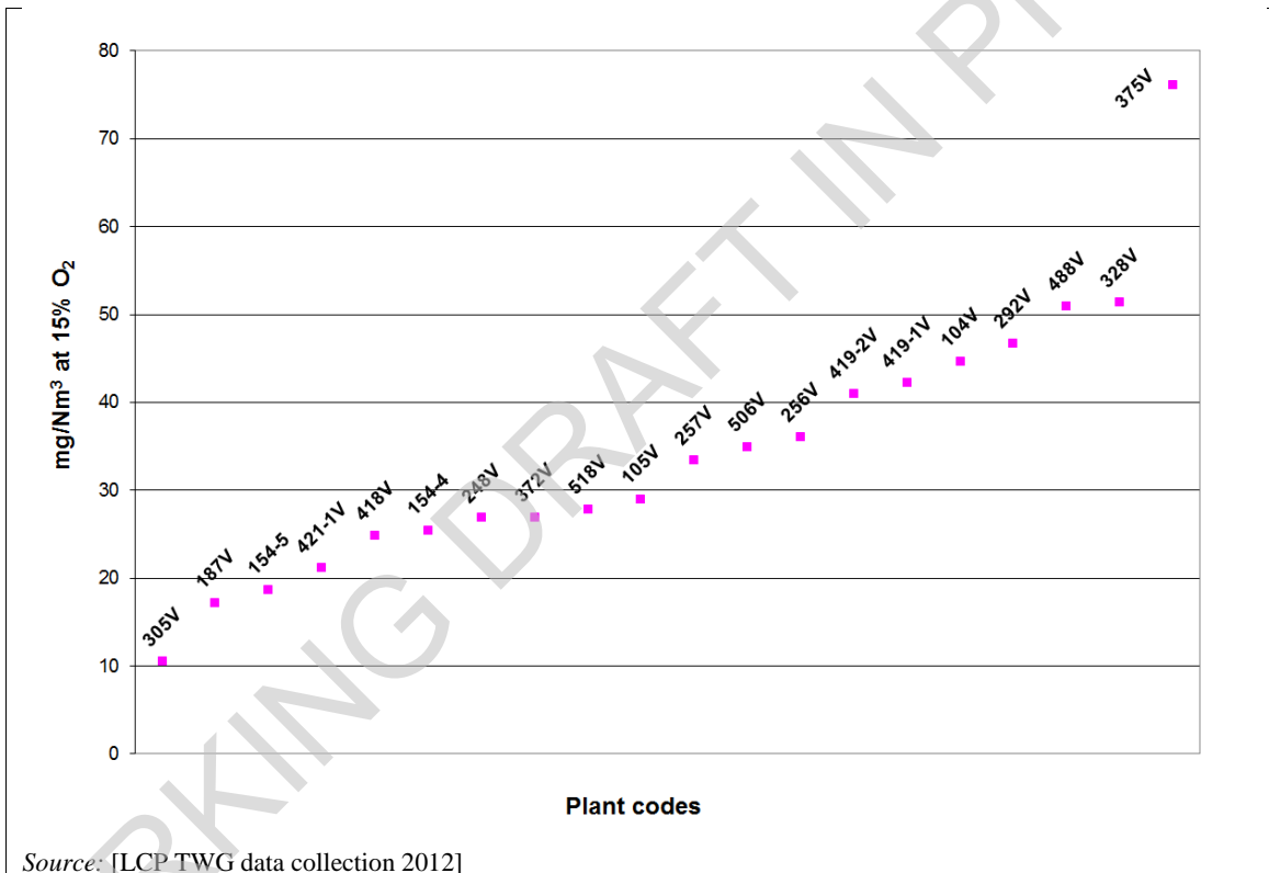
Figure 7.14: NO x emissions (yearly averages) from CCGTs fitted with supplementary firing at the HRSG level
