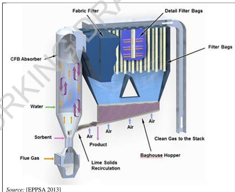
Figure 3.25: Schematic of a CFB scrubber process flow
