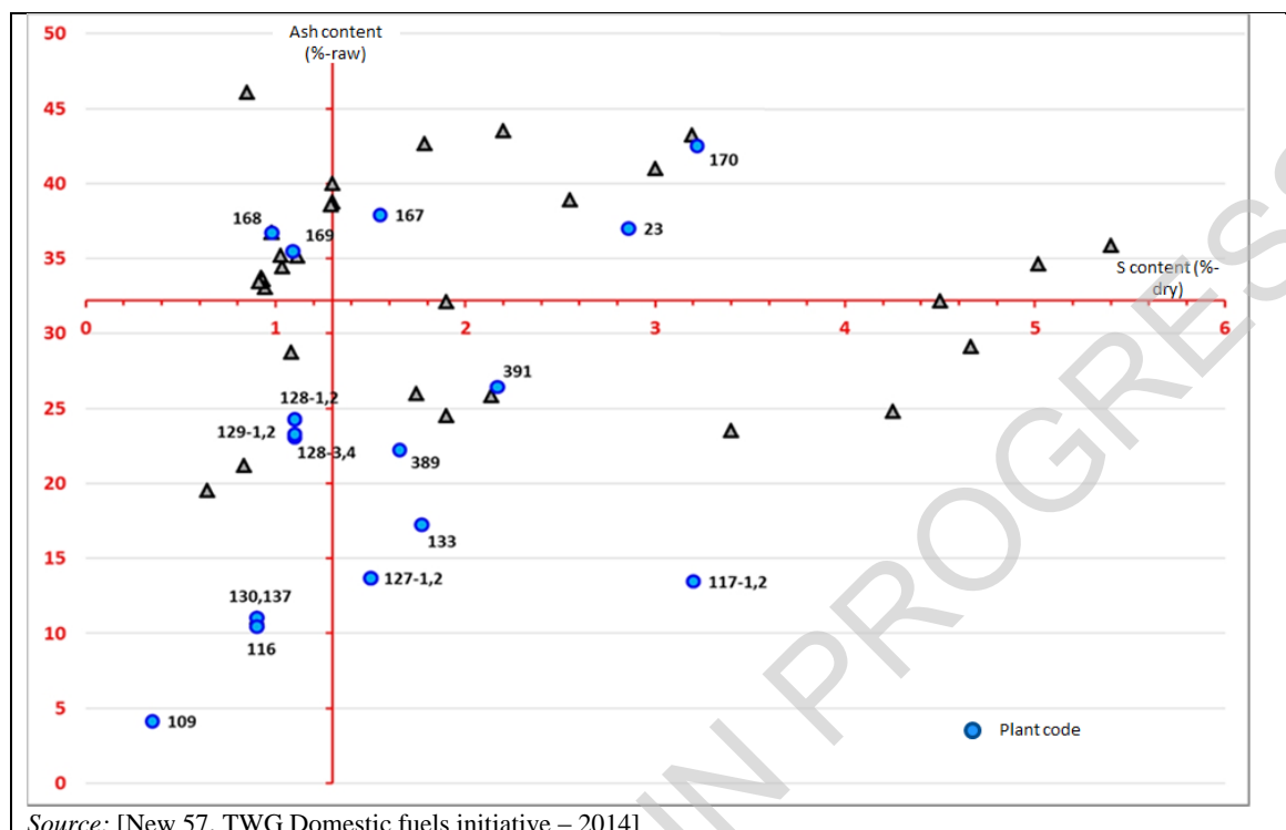
Figure 5.11: Sulphur and ash content in EU lignites ([wt-%], cross in medians)
