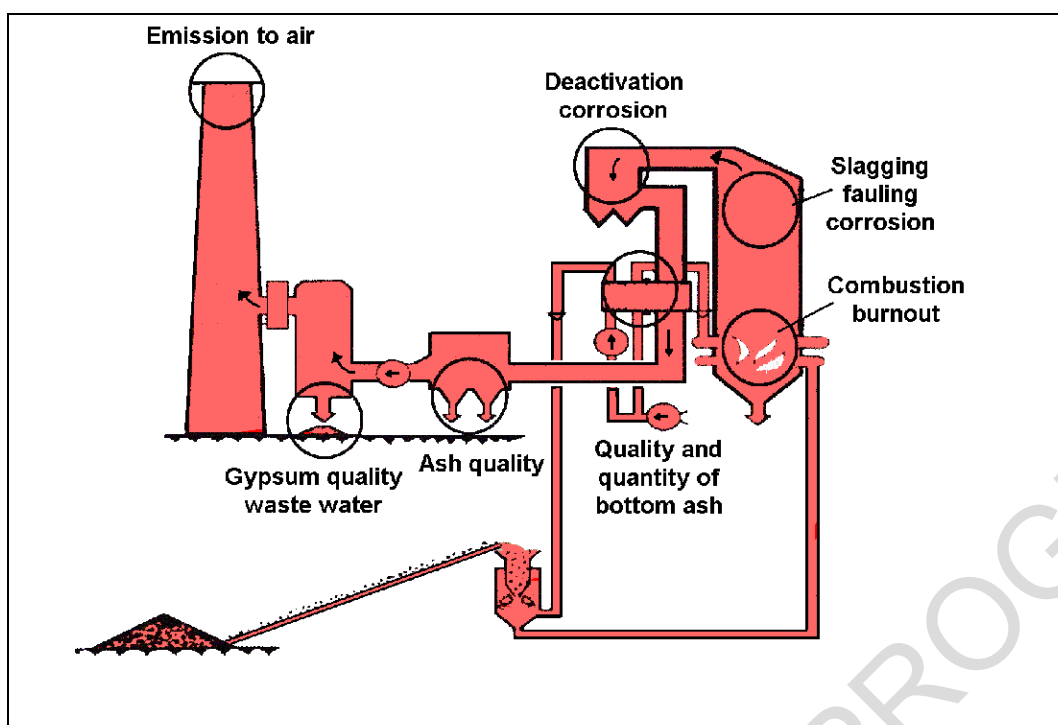
Figure 5.6: Influence of coal quality on the performance of the combustion plant
