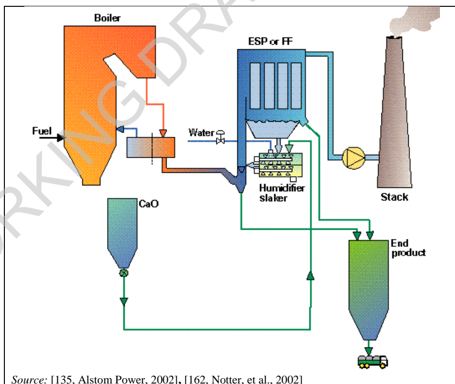
Figure 3.27: 'Modified dry FGD' process
