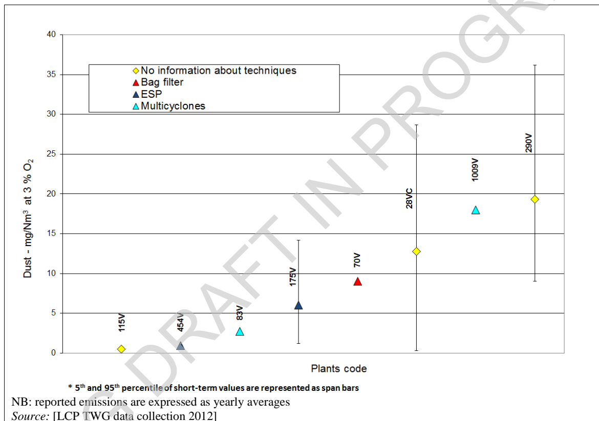
Figure 6.7: Dust emissions from well-performing HFO- and/or gas-oil-fired boilers of < 300 \text{ MW}_{\text{th}}
