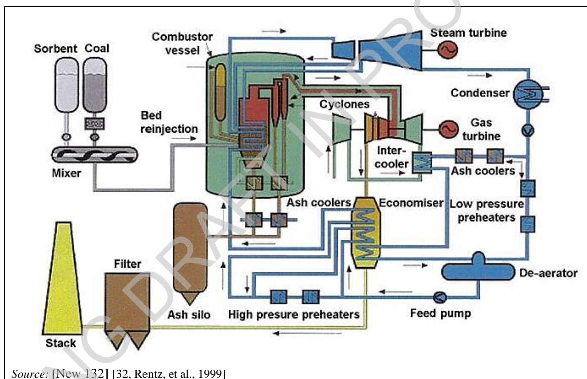
Figure 2.8: Schematic drawing of a bubbling bed PFBC system
