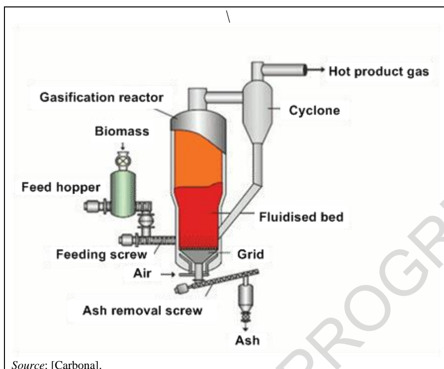
Figure 4.9: ANDRITZ Carbona air-blown pressurised BFB gasifier
