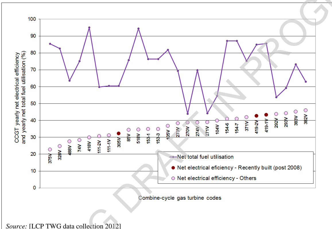
Figure 7.18: Typical net operating energy efficiencies in 2010 of European natural-gas-fired combined-cycle gas turbines producing heat and power (plants from 50 MW th to 600 MW th )
