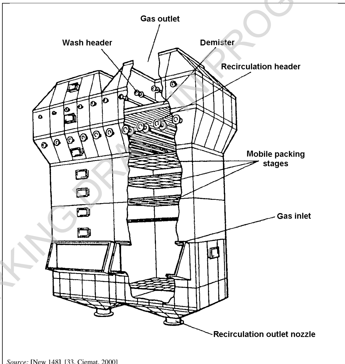
Figure 3.17: Moving-bed scrubber
