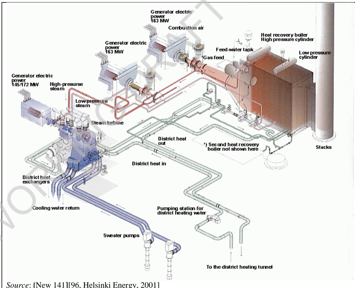
Figure 2.20: Gas turbine combined-cycle power plant
