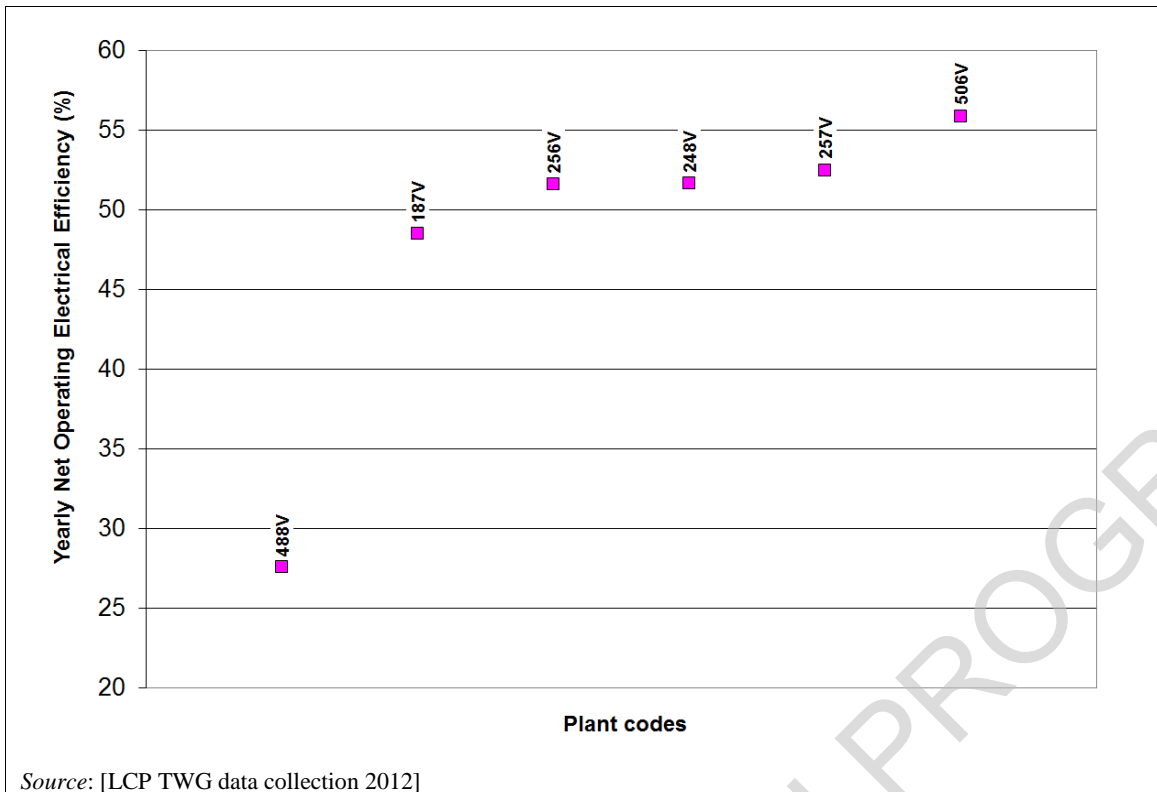
Figure 7.6: Net operating electrical efficiencies of CCGTs with supplementary firing in 2010
