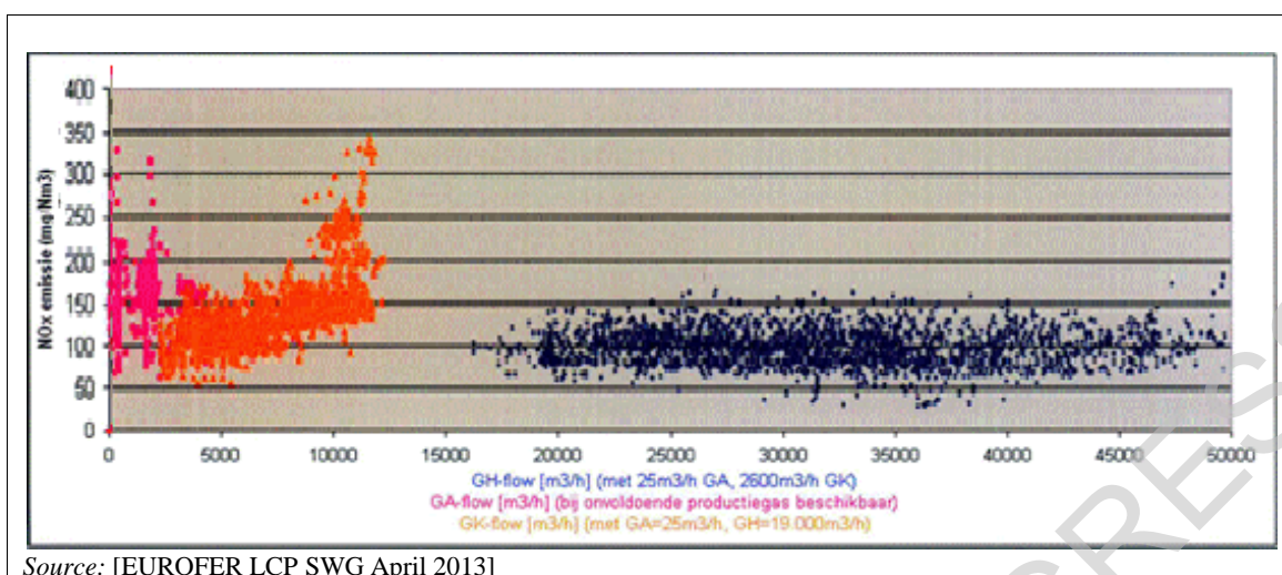
Figure 7.45: NO x emissions (mg/Nm 3 ) against the gas flows (m 3 /h) for a boiler using three different base gas mixes
