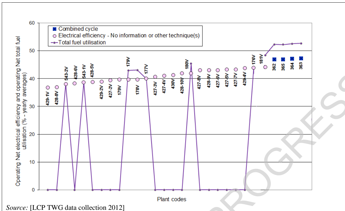
Figure 6.9: Operating energy efficiencies of European HFO- and/or gas-oil-fired combustion engines
