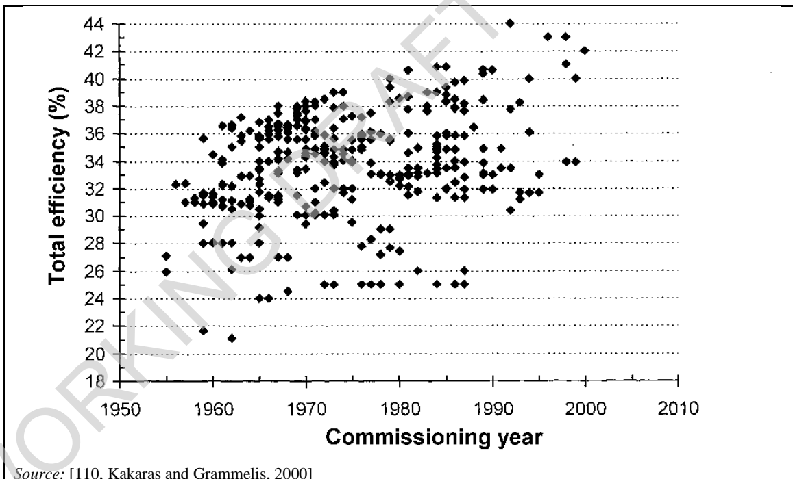
Figure 5.13: Efficiency of coal-fired power plants in Europe in relation to the commissioning year based on design values
