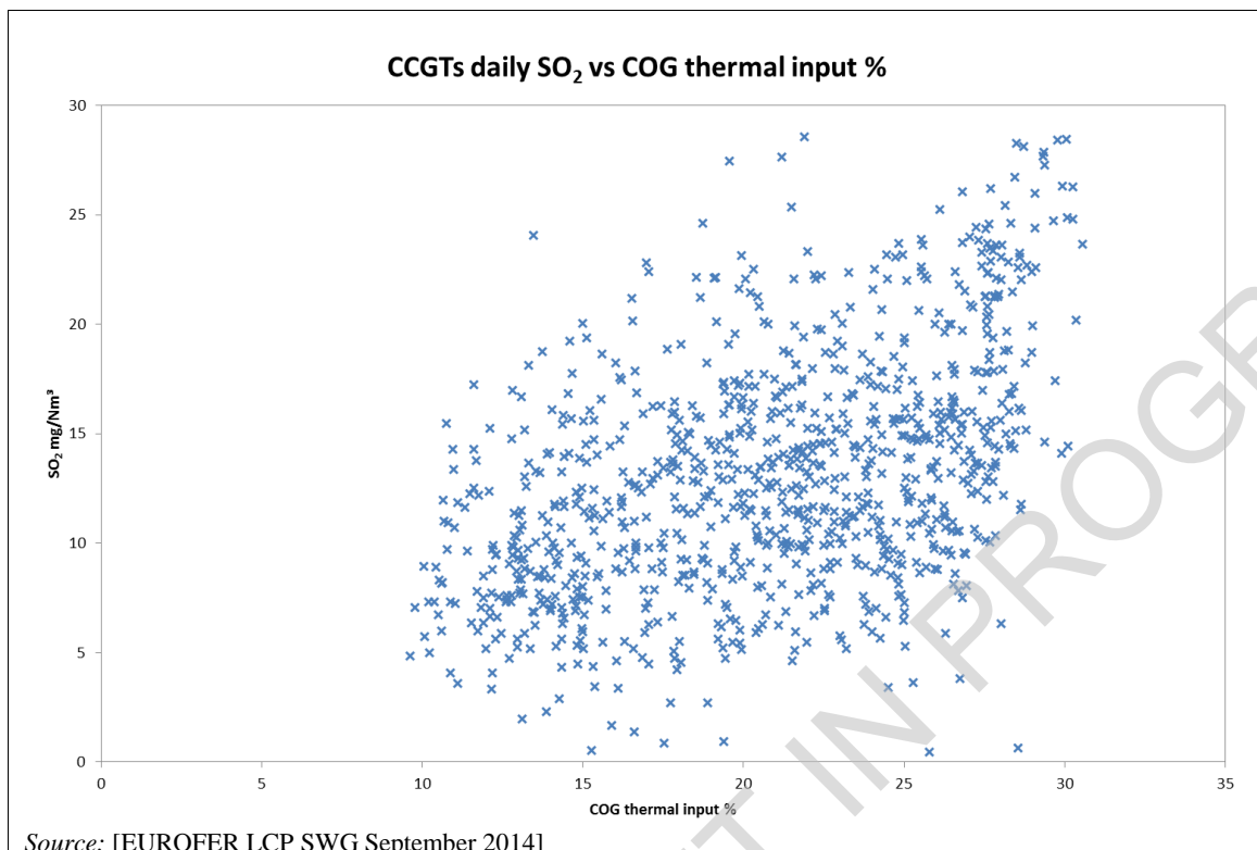
Figure 7.48: Relationship between SO 2 emissions and the inputs to 3 CCGTs from COG using daily average data for 2010
