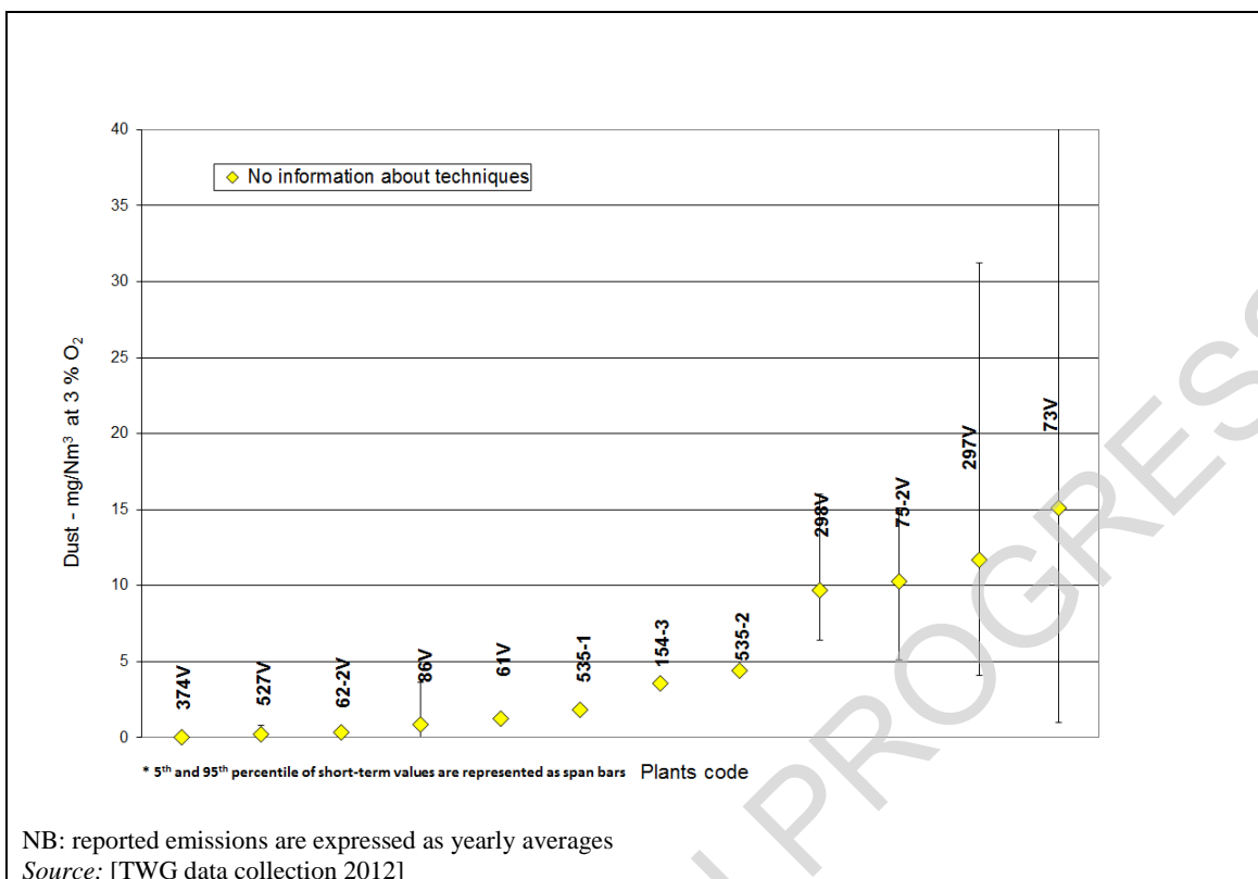
Figure 8.11: Dust emissions from example plants firing mixtures of process gaseous and liquid fuels from the chemical industry
