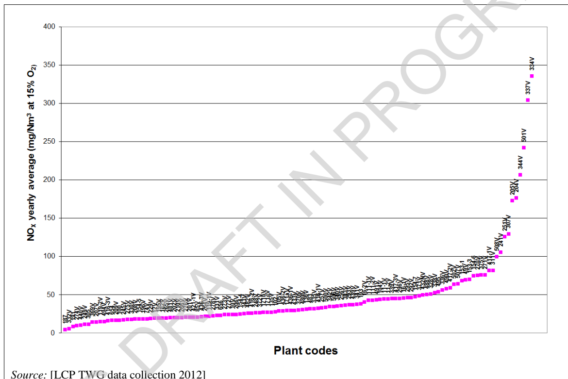
Figure 7.11: \text{NO}_x emissions from European natural-gas-fired turbines in 2010
