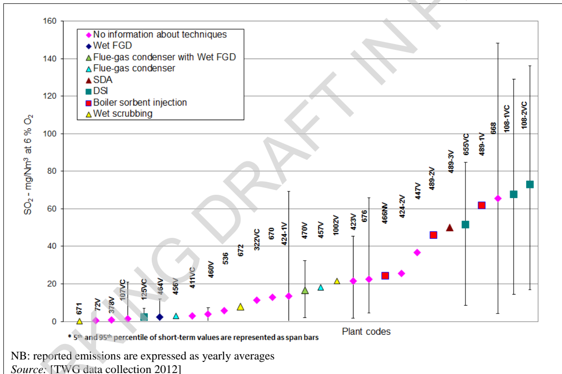
Figure 5.48: SO 2 emissions from well-performing biomass- and/or peat-fired plants of < 100 MW th
