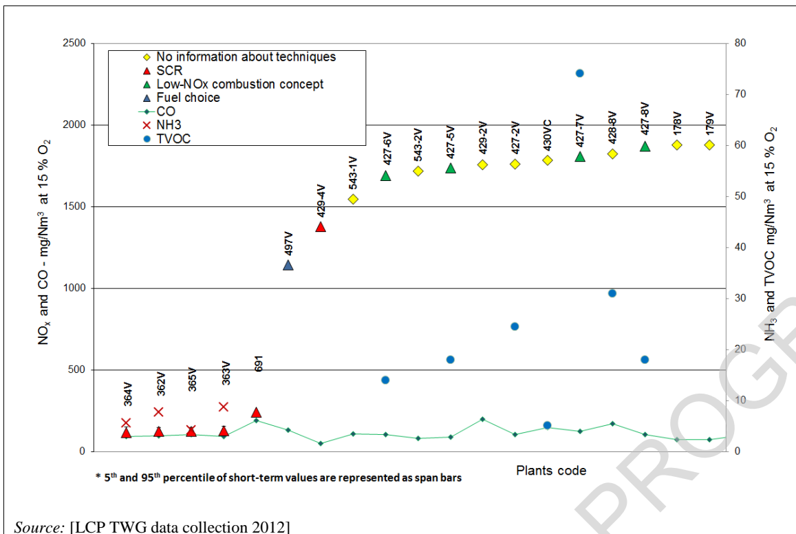
Figure 6.11: Yearly NO x emissions from HFO- and/or gas-oil-fired engines fitted with SCR and/or primary techniques
