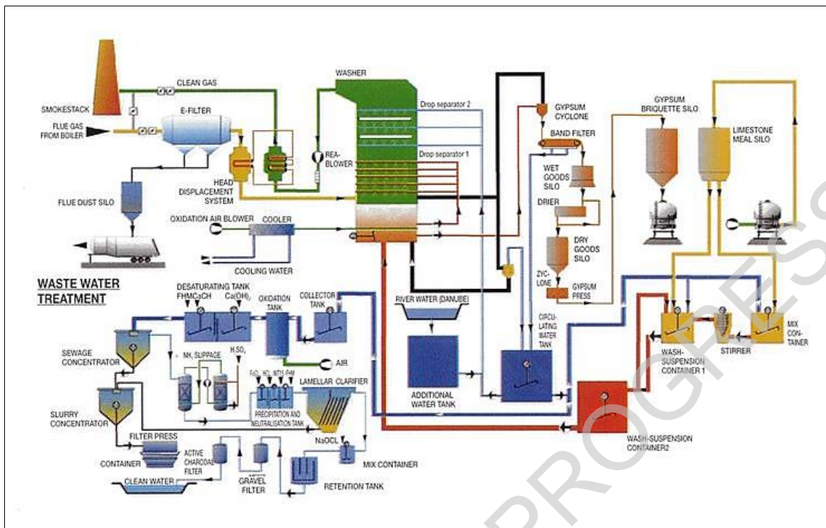
Figure 6.4: Wet FGD process applied to a HFO-fired boiler
