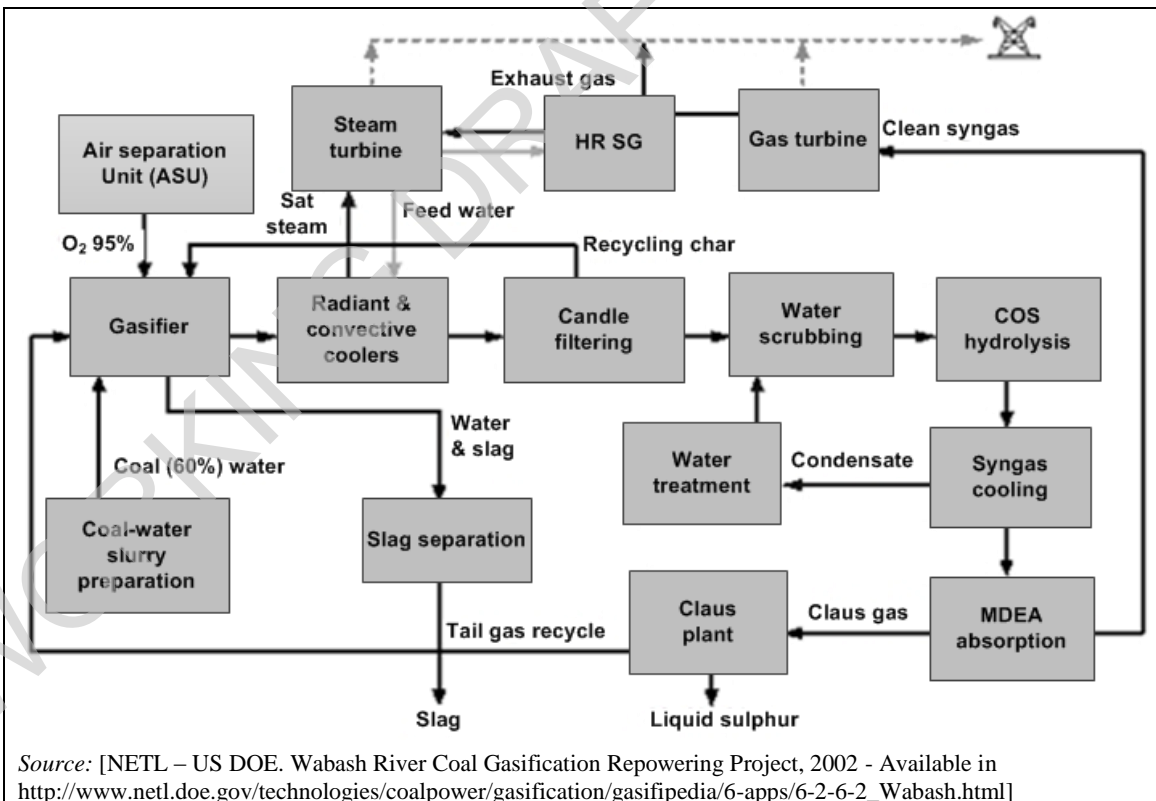
Figure 4.6: Block diagram of the Wabash River IGCC repowering project
