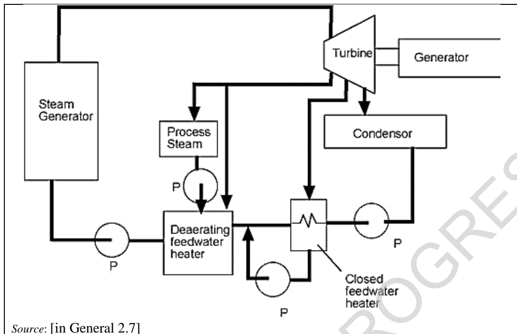
Figure 3.54: Feed-water preheating
