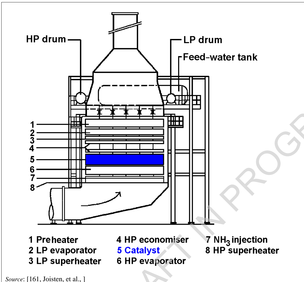
Figure 7.3: SCR installation with vertical flow
