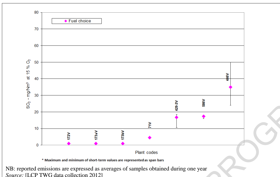
Figure 6.16: SO 2 emissions from well-performing gas-oil-fired gas turbines
