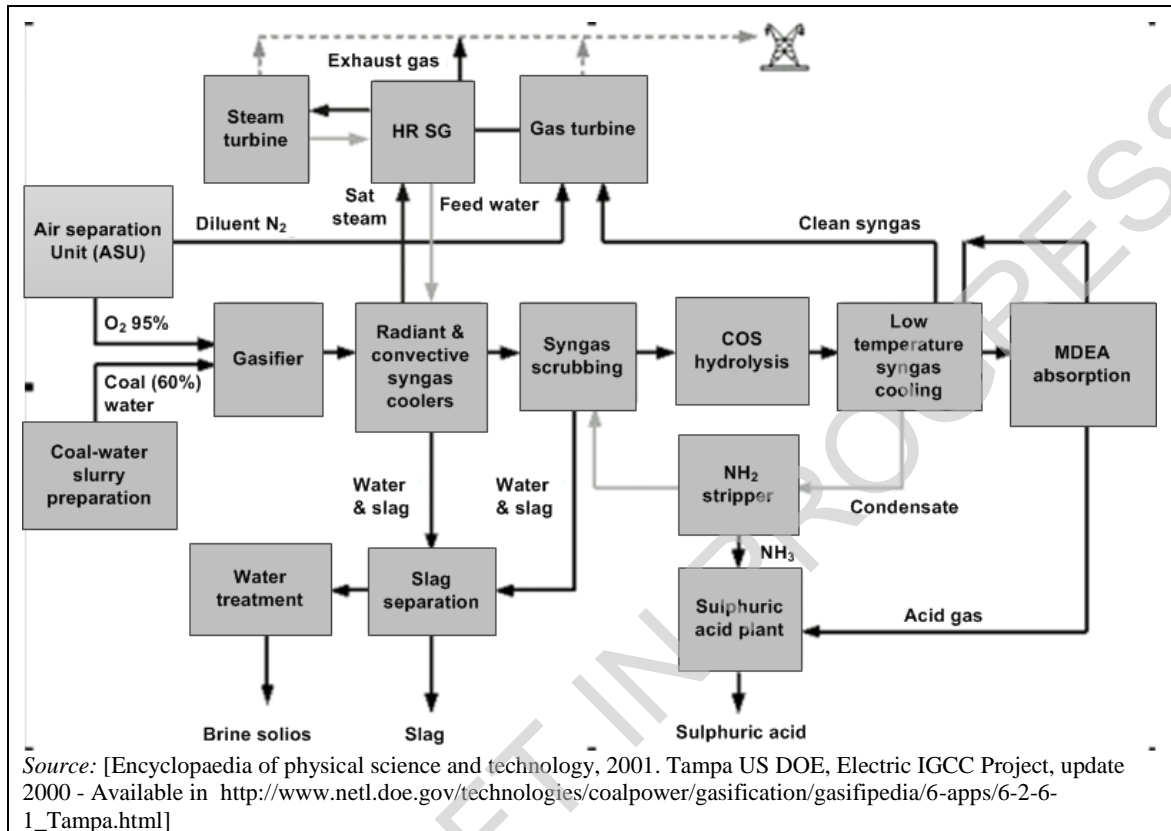
Figure 4.4: Block diagram of the Tampa IGCC plant process
