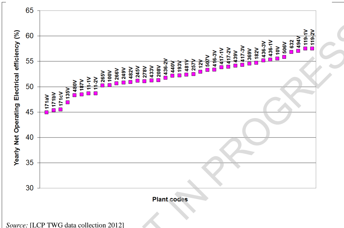
Figure 7.8: Net operating electrical efficiencies of CCGTs producing only power operated \geq 4000 hours in 2010
