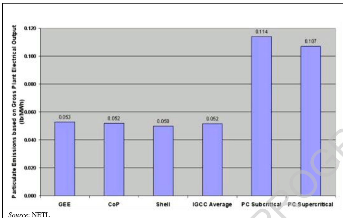
Figure 4.13: Particulate emissions of currently feasible coal-to-electricity technology options without CO 2 capture
