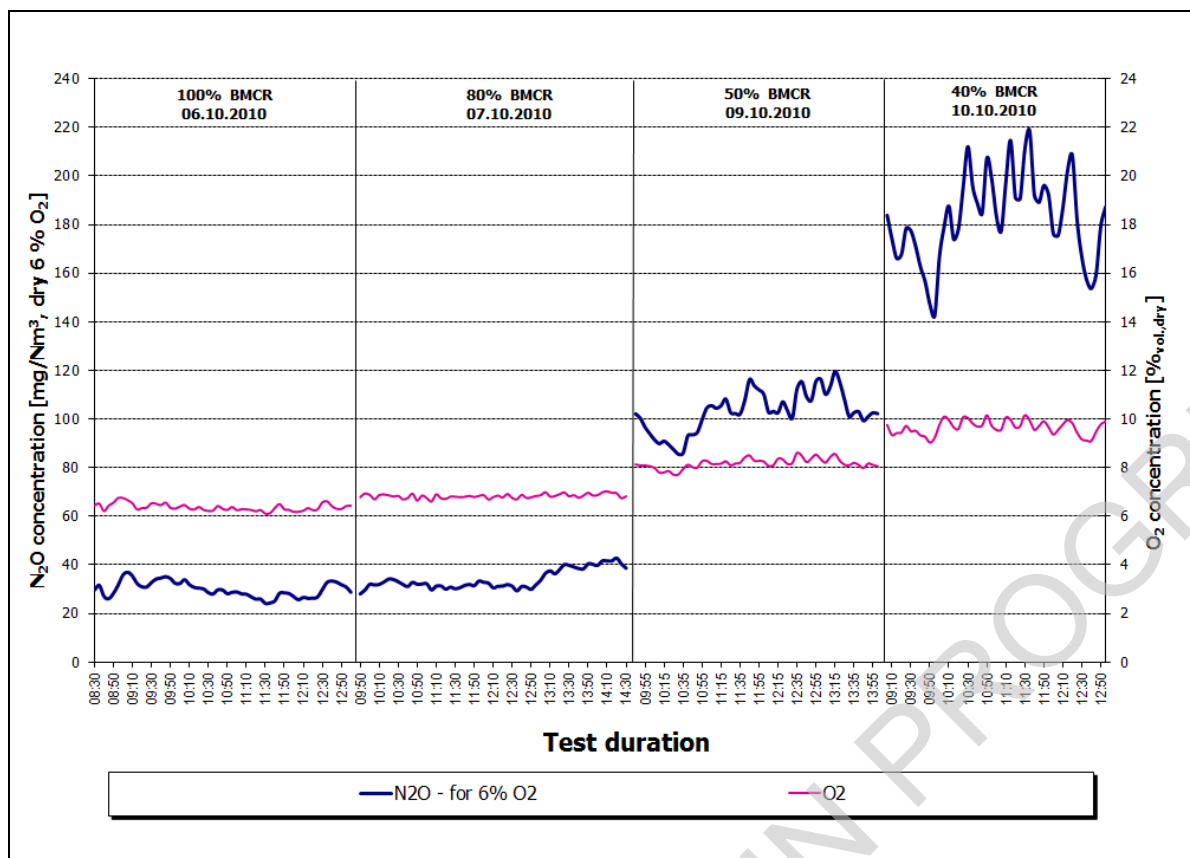
Figure 5.18: Impact of the equivalent full load factor on N_2O emissions at Plant 387 (Lagisza, PL)
