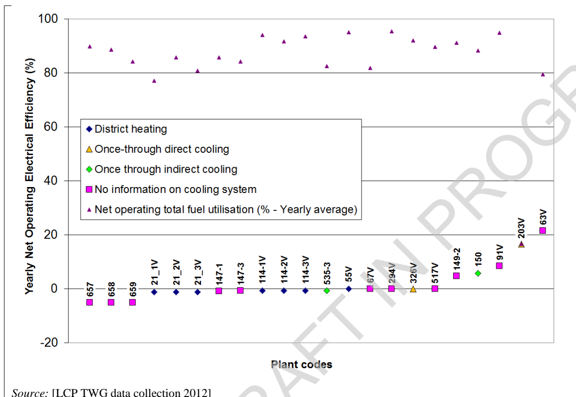
Figure 7.10: Net operating electrical efficiencies and total fuel utilisation in 2010 of natural-gas-fired boilers
