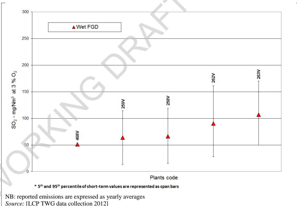
Figure 6.6: SO 2 emissions from well-performing HFO- and/or gas-oil-fired boilers of ≥ 300 MW th
