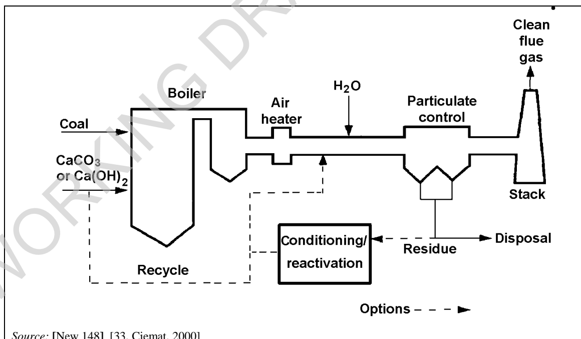
Figure 3.28: Furnace sorbent injection
