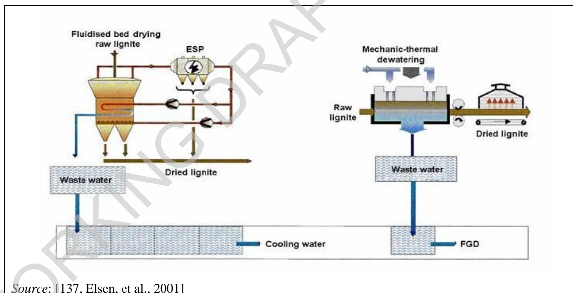
Figure 11.5: Pilot plant for lignite drying
