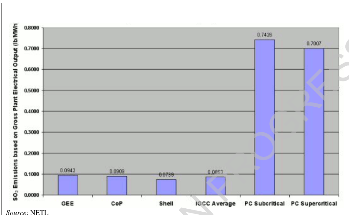
Figure 4.11: SO 2 emissions of currently feasible coal-to-electricity technology options without CO 2 capture
