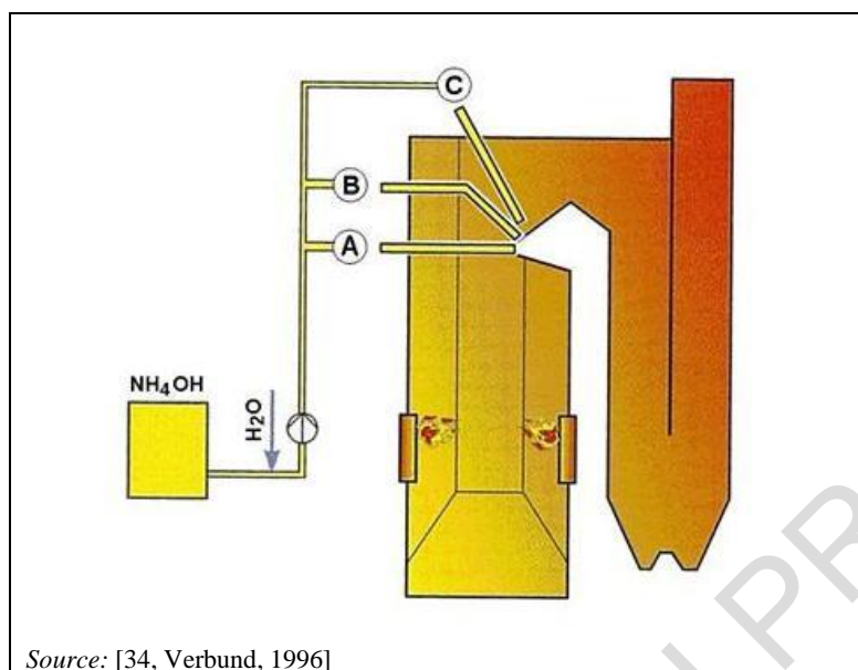
Figure 3.47: The SNCR process
