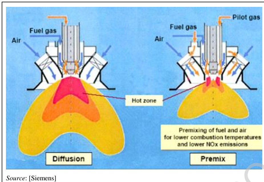
Figure 3.39: Schematic of a DLN (premix) combustion chamber
