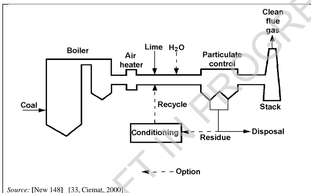
Figure 3.26: Duct sorbent injection
