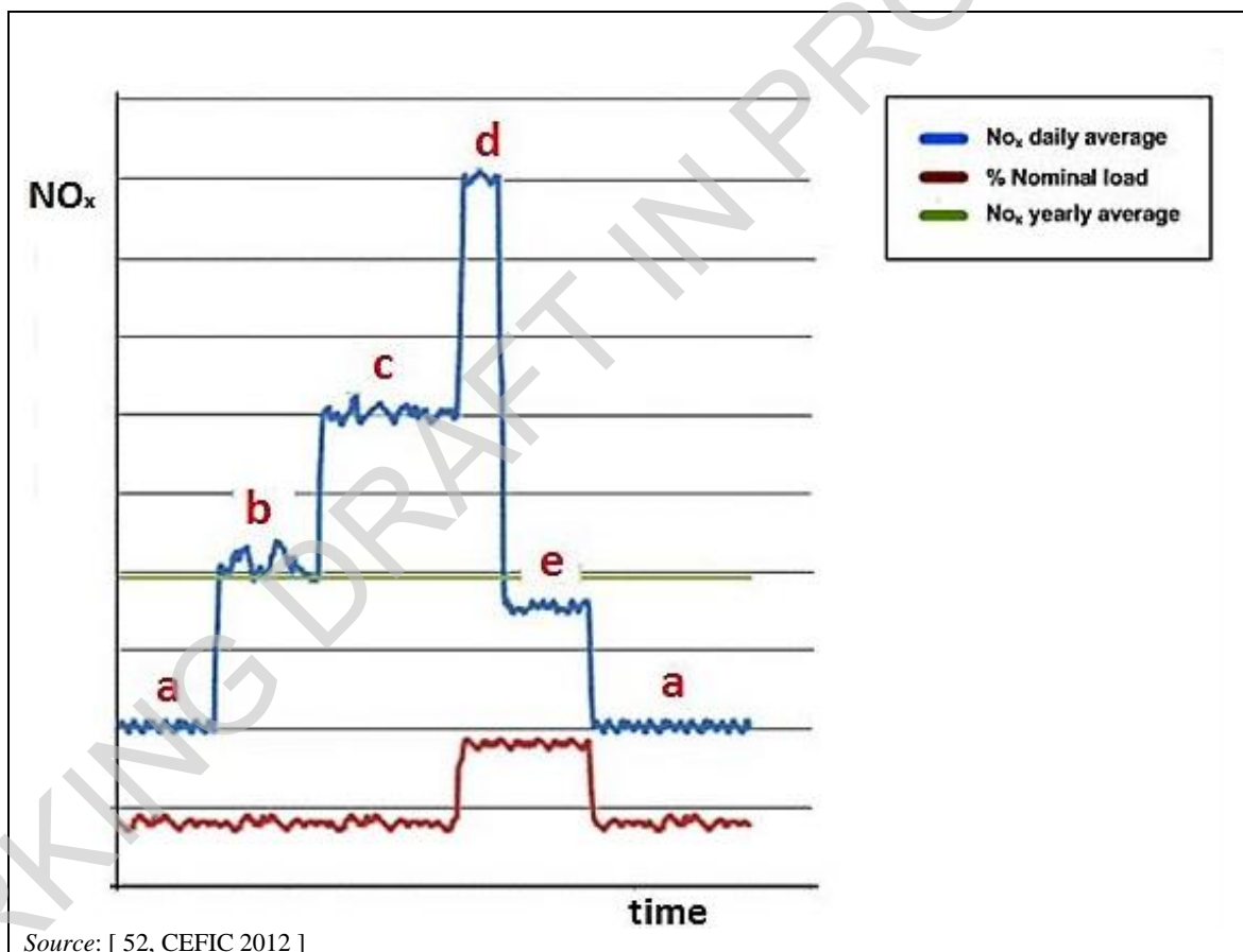
Figure 8.4: NO x emissions pattern as a function of the daily operation of a utility boiler not fitted with end-of-pipe measures (values are not taken from real installations)
