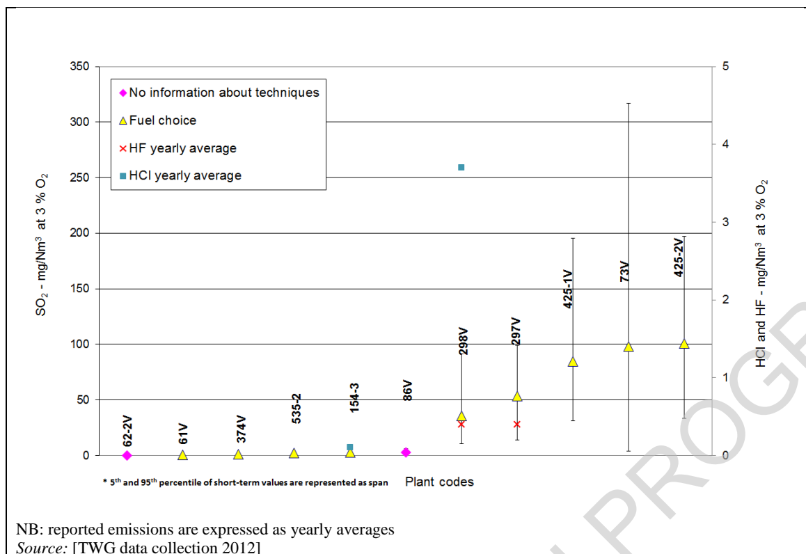
Figure 8.10: SO 2 , HCl and HF emissions from example plants firing mixtures of process gaseous and liquid fuels from the chemical industry
