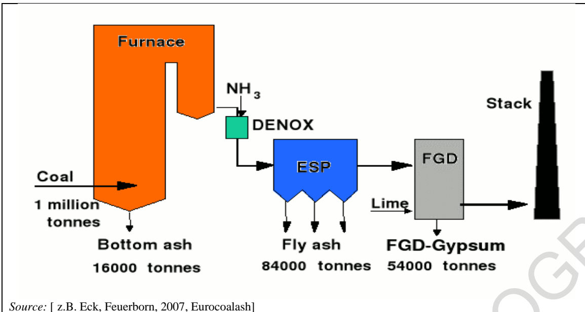
Figure 5.19: Annual production of CCPs in a 450 MW e coal-fired power plant at 6000 hours full load (total production of CCPs = 187 000 tonnes)
