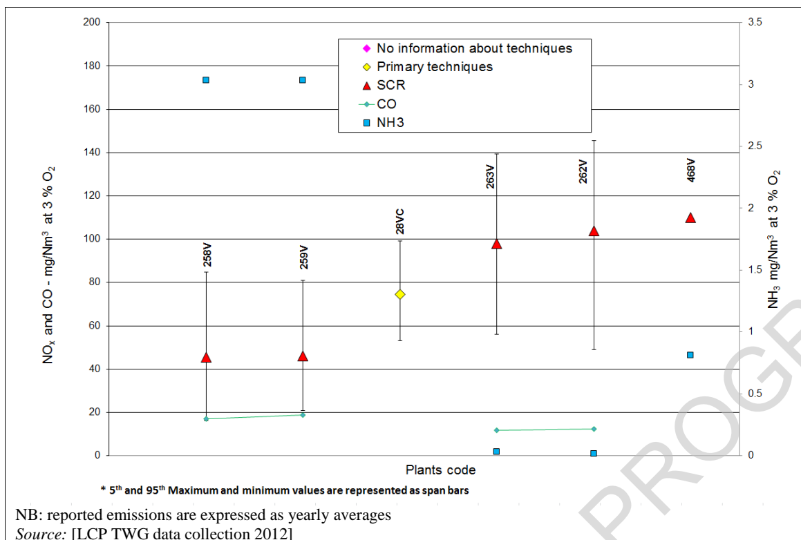
Figure 6.3: NO x emissions from well-performing HFO- and/or gas-oil-fired boilers of \geq 100 \text{ MW}_{th}
