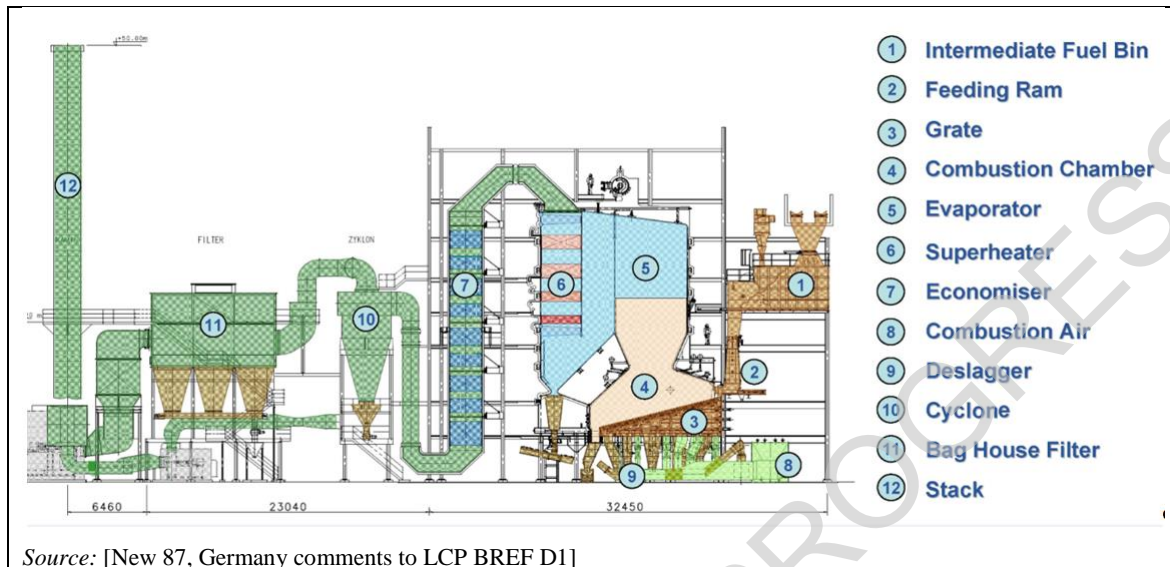
Figure 5.39: Water-cooled vibrating moving grate system with sloped grate boiler for biomass combustion
