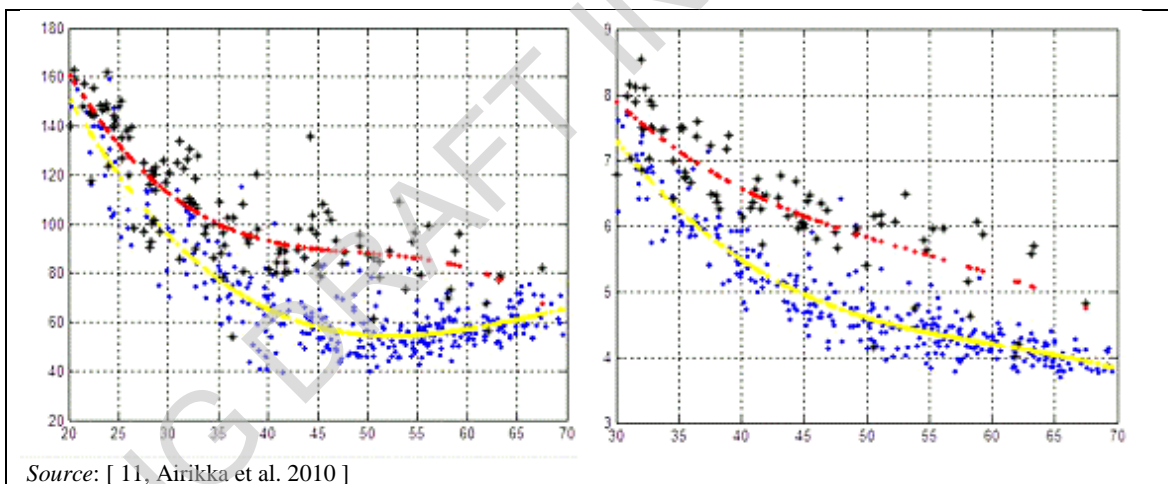
Figure 3.11: Example of NO x (left) (mg/Nm 3 ) and O 2 (right) (%) (y axis) for different load factors (x axis) at a BFB boiler in Sweden
