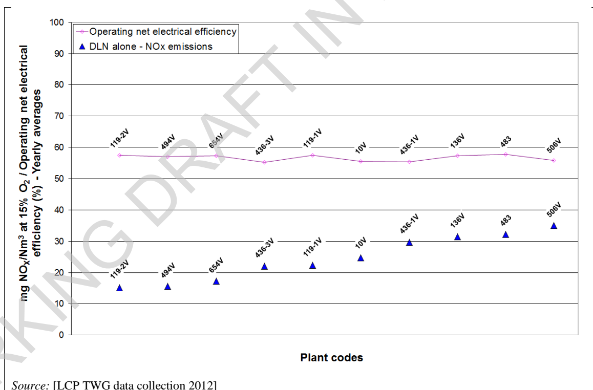
Figure 7.13: Example of CCGTs achieving low NO x emissions and high operating electrical efficiencies
