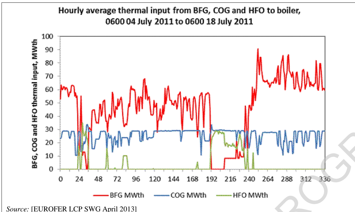
Figure 7.38: Hourly average thermal inputs of BF gas, COG and HFO to a boiler over a two-week period
