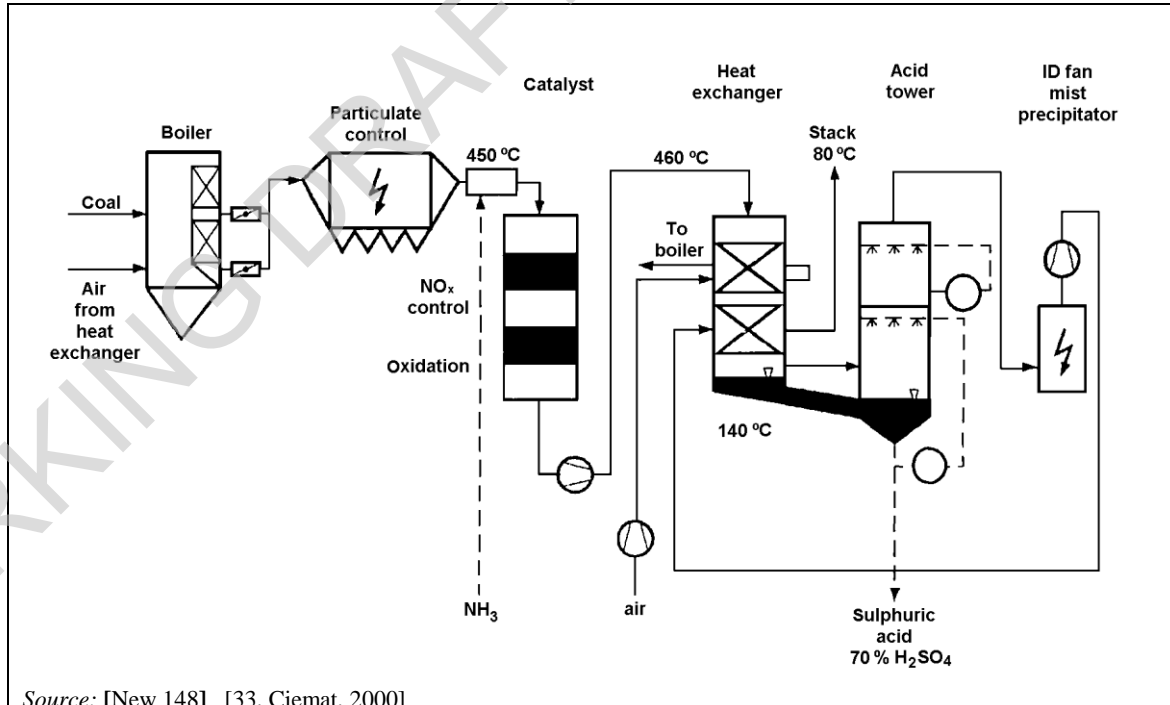
Figure 3.50 The DeSONO x process
