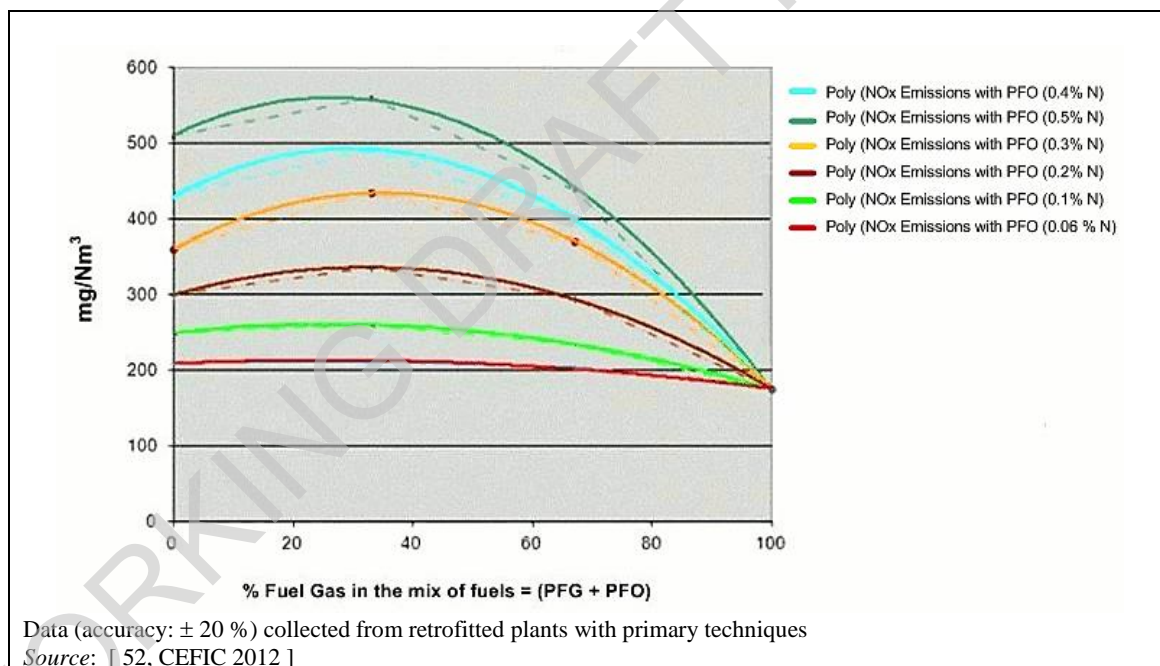
Figure 8.5: NO_x concentration pattern in raw flue-gas as a function of the fuel blend at nominal load
