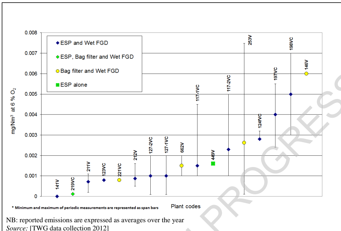
Figure 9.4: Cd+Tl emissions from well-performing coal- and lignite-fired plants of more than 300 MW th , including plants co-incinerating waste (averages over the year)
