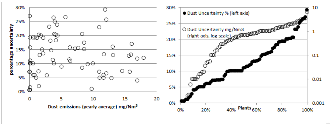
Figure 13.3: Measurement uncertainties reported for dust emissions
