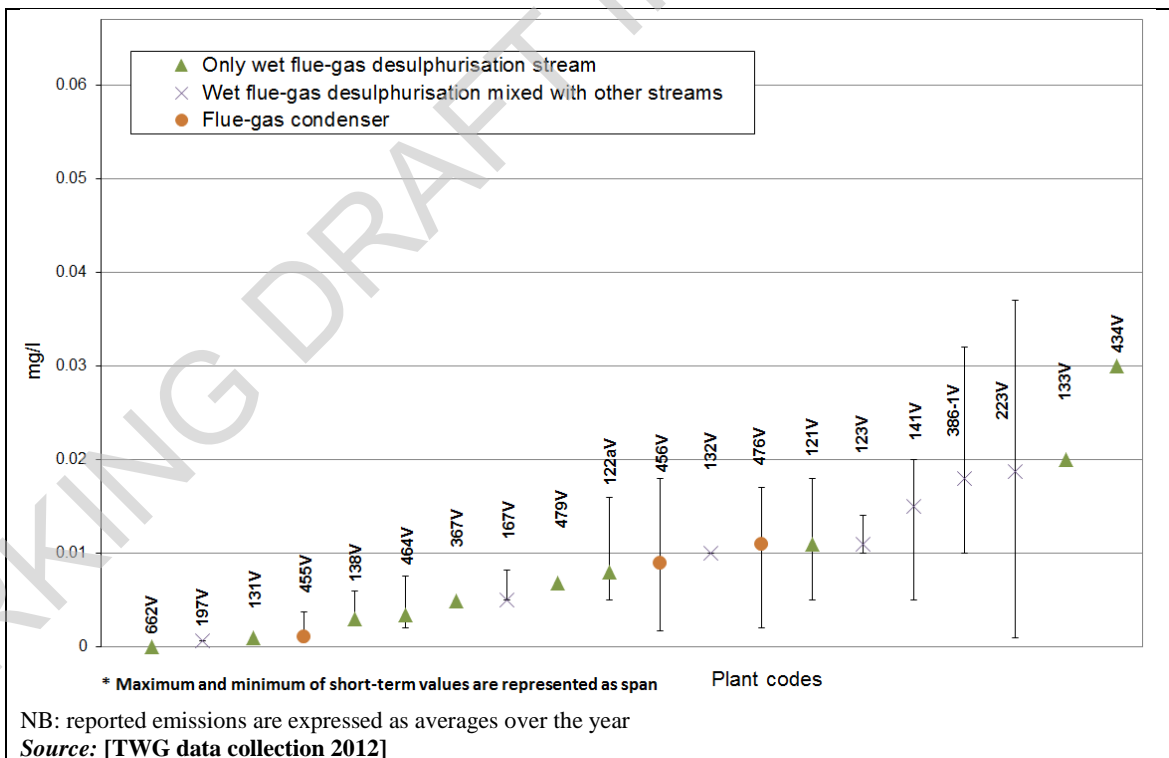
Figure 3.68: Copper (Cu) emissions in direct discharges to a receiving water body
