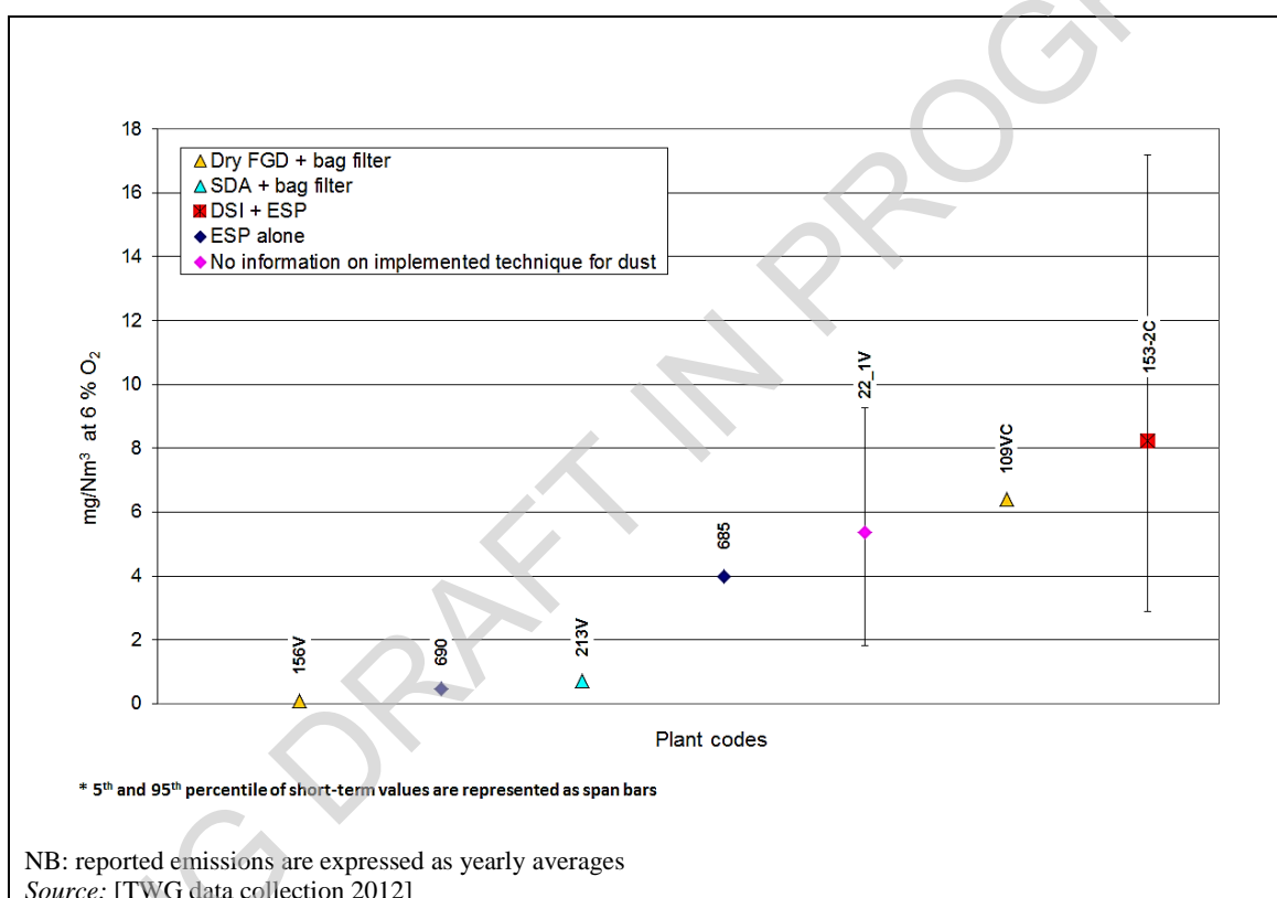
Figure 5.27: Yearly average dust emissions from well-performing coal- and/or lignite-fired plants sized between 100 MW th and 300 MW th
