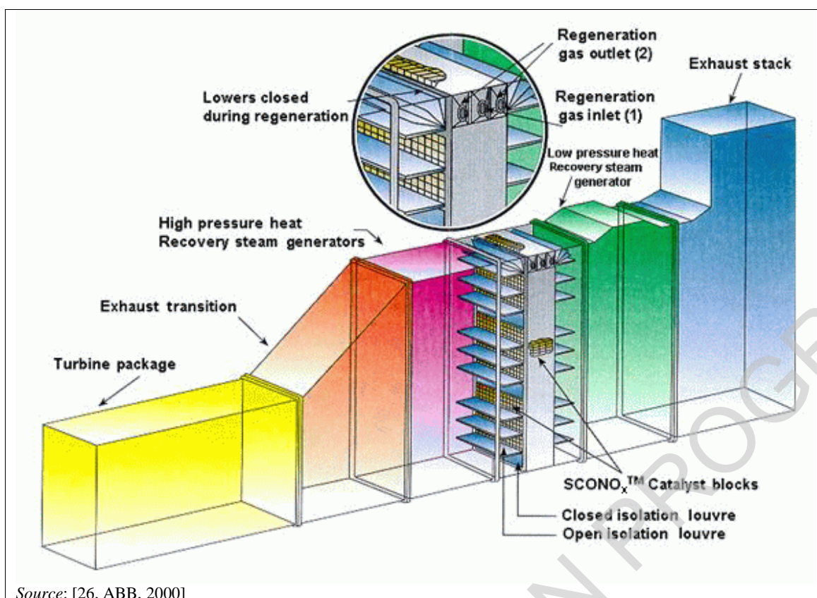
Figure 7.31: Schematic representation of the catalyst pollution control SCONO x TM system
