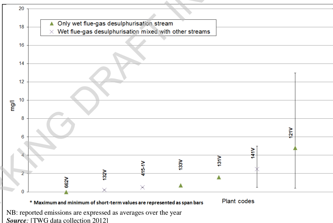
Figure 3.64: Sulphite ( SO_3^{2-} ) emissions in direct discharges to a receiving water body
