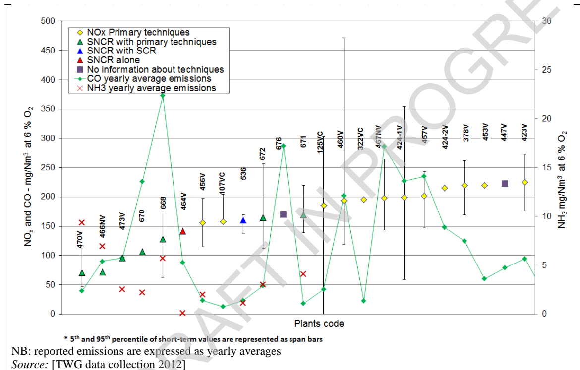
Figure 5.45: \text{NO}_x emissions from well-performing biomass- and/or peat-fired plants of < 100 \text{MW}_{\text{th}}
