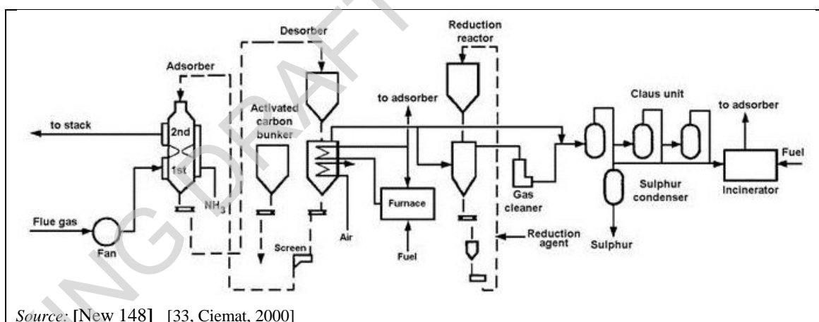
Figure 3.48: The activated carbon process
