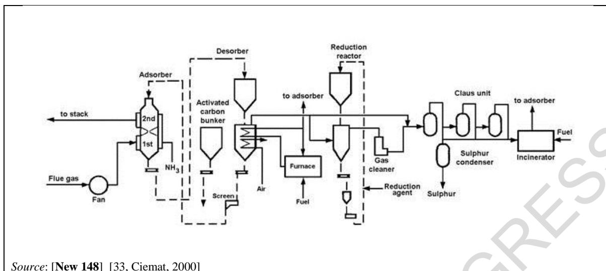
Figure 3.4 The activated carbon process
