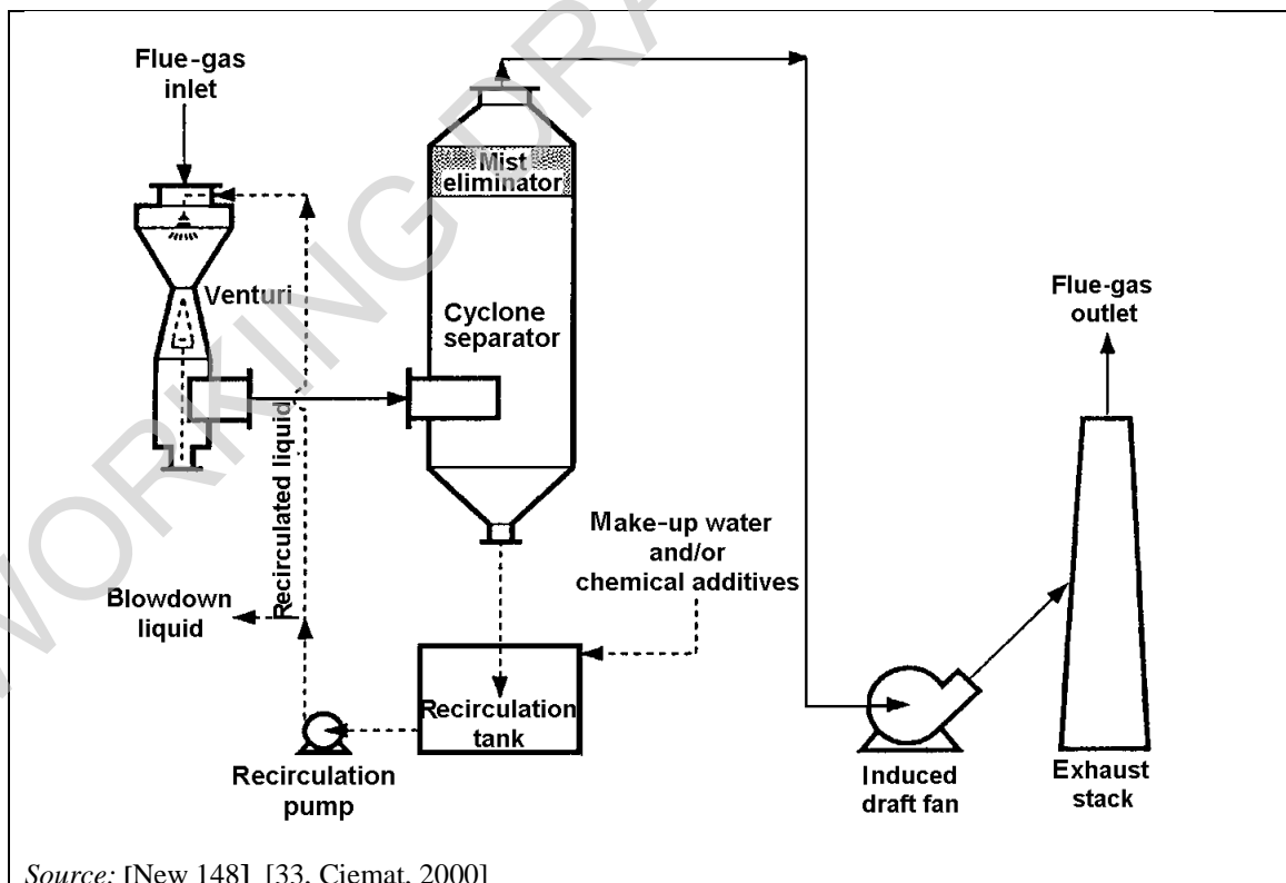
Figure 3.16: Typical flow diagram of a venturi system
