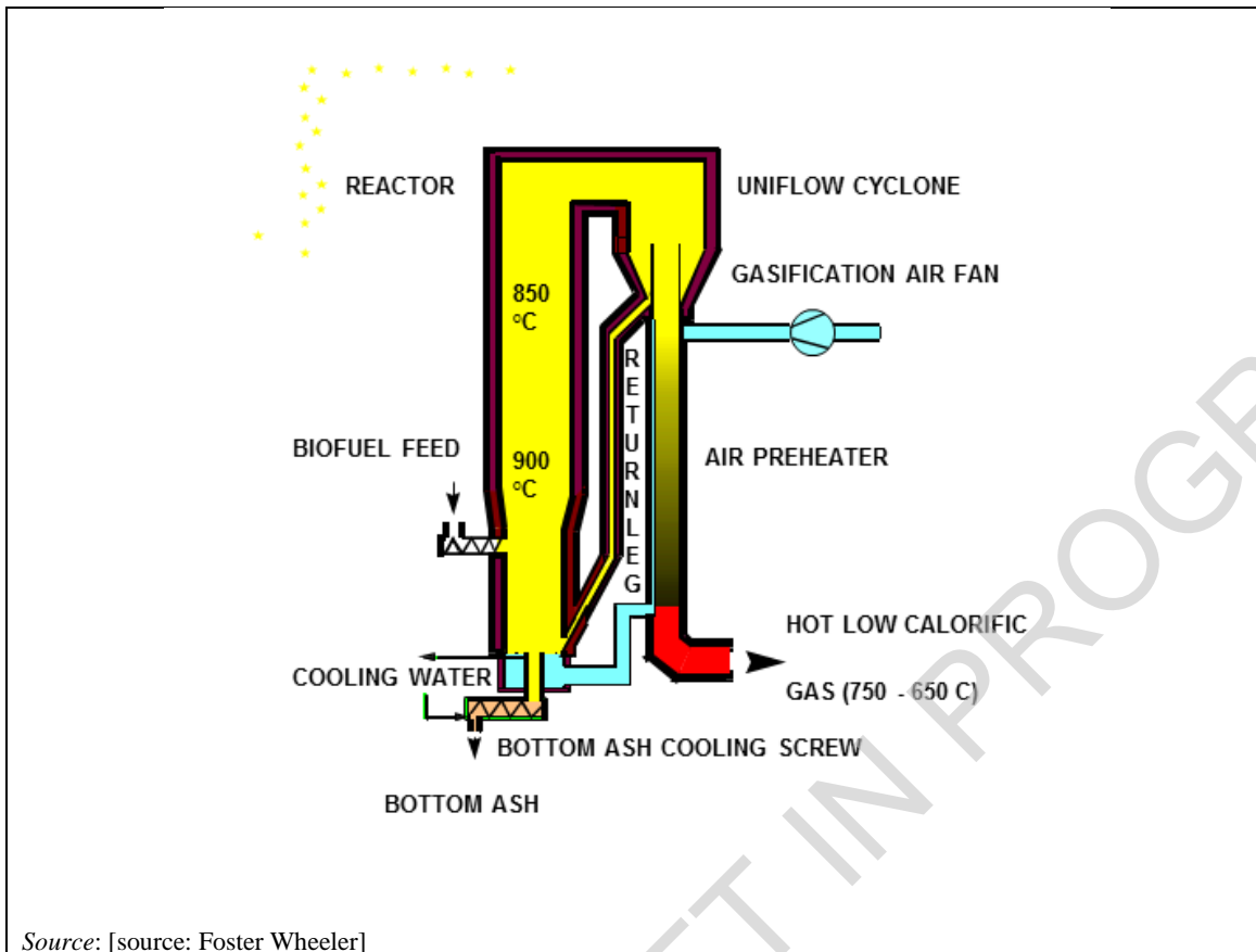
Figure 4.8: Foster and Wheeler atmospheric CFB gasifier
