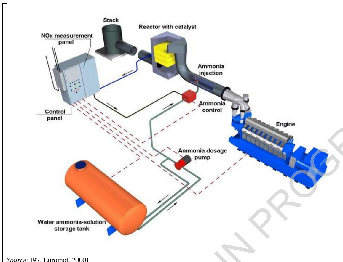
Figure 3.45: SCR system applied to a stationary combustion engine
