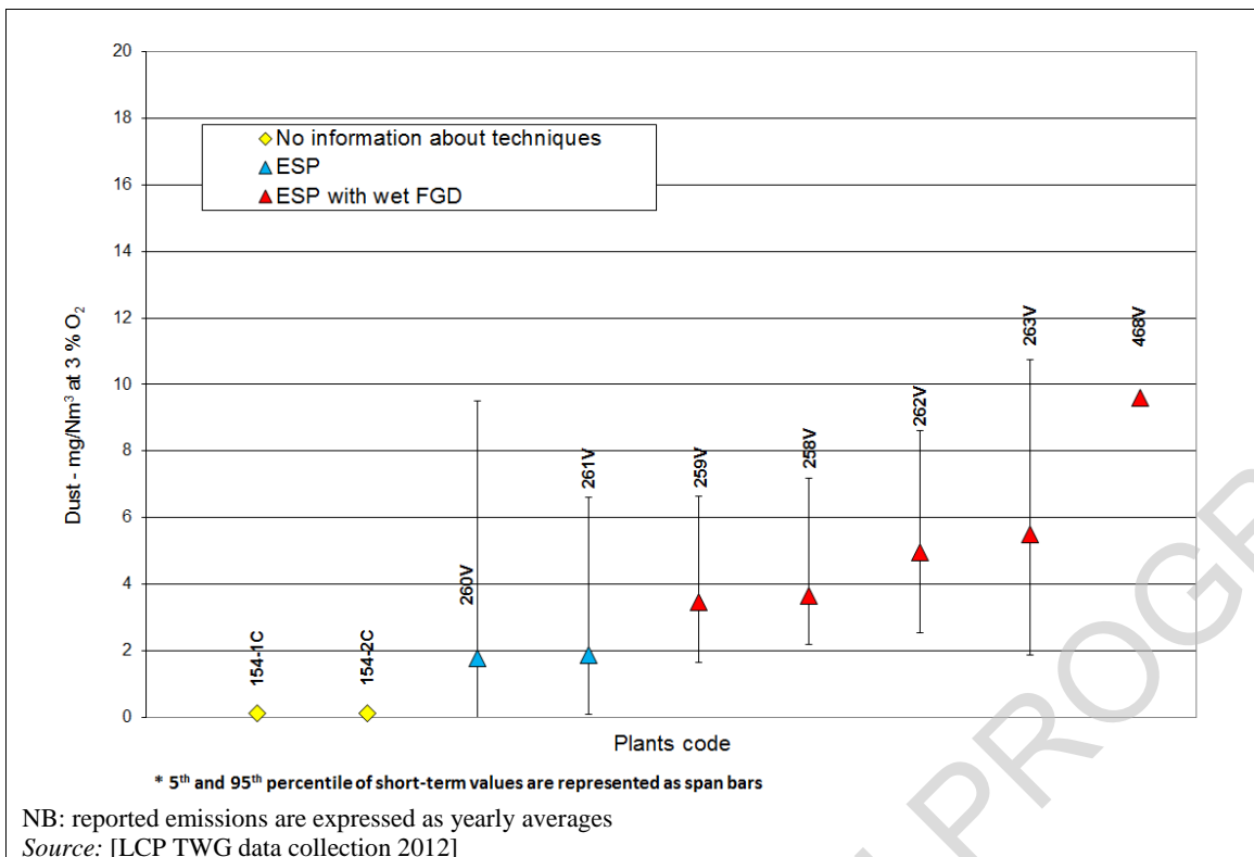
Figure 6.8: Dust emissions from well-performing HFO- and/or gas-oil-fired boilers of \geq 300 \text{ MW}_{\text{th}}
