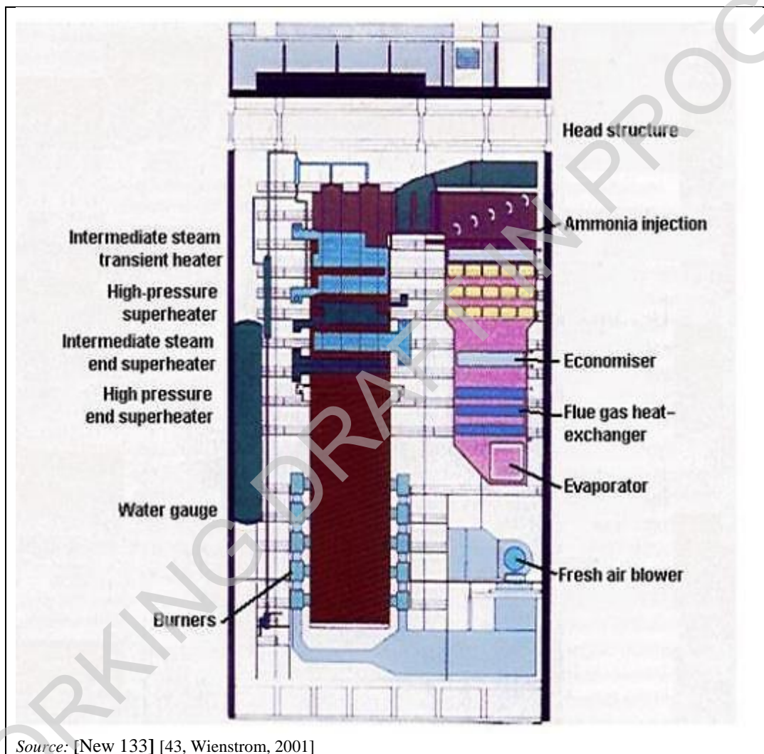
Figure 2.3: Heavy fuel oil boiler
