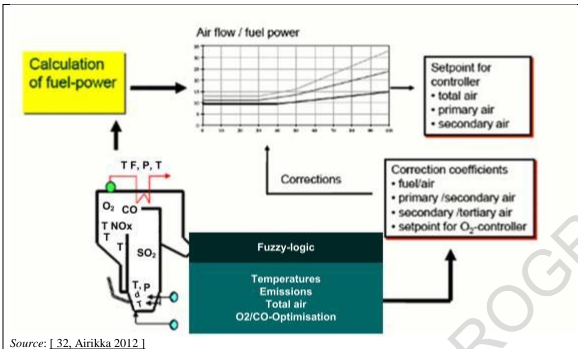
Figure 3.55: Advanced control system applied at the Billerud AB Karlsborg plant, Sweden
