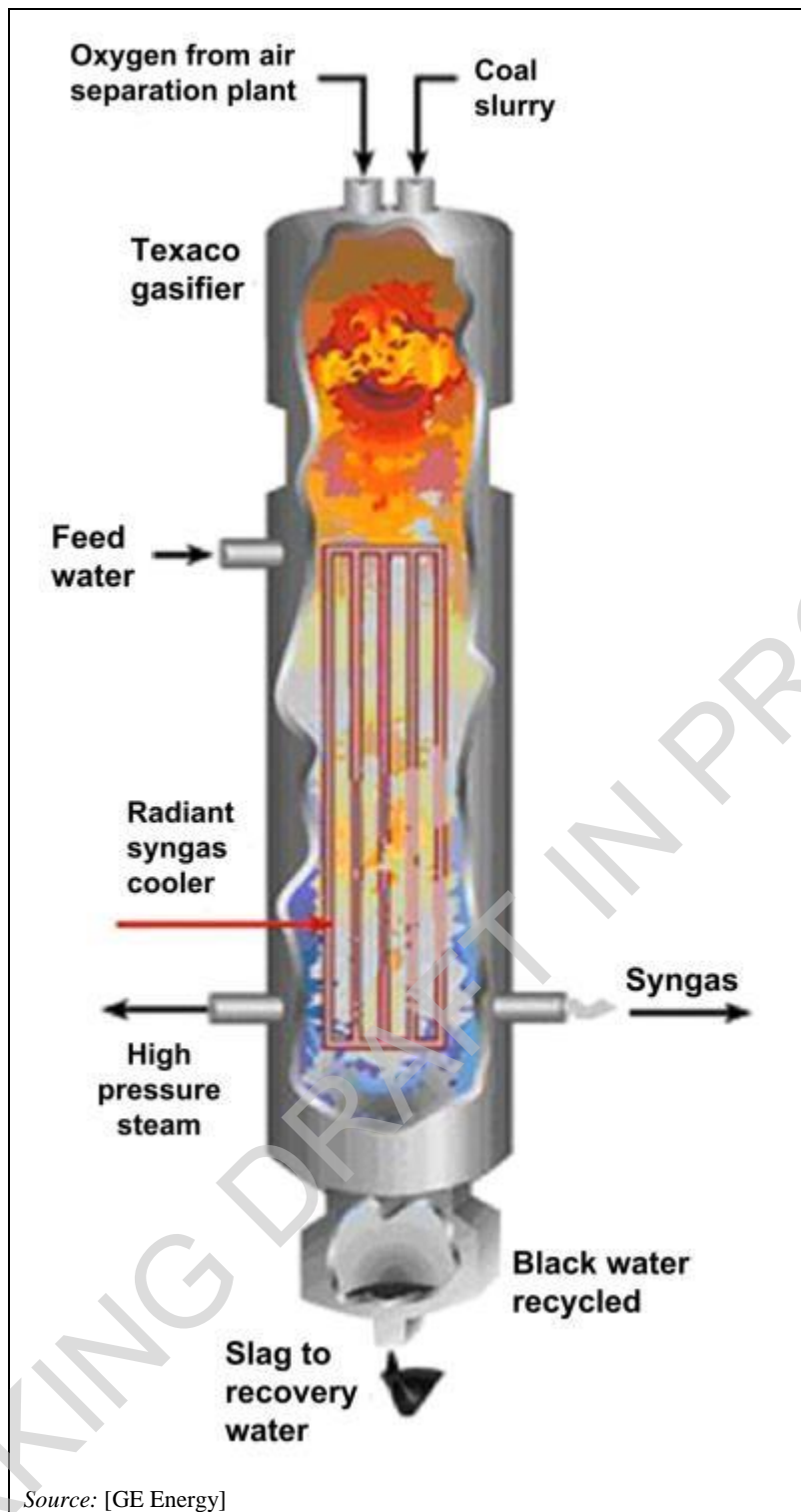
Figure 4.2: General Electric single-stage entrained-flow gasifier
