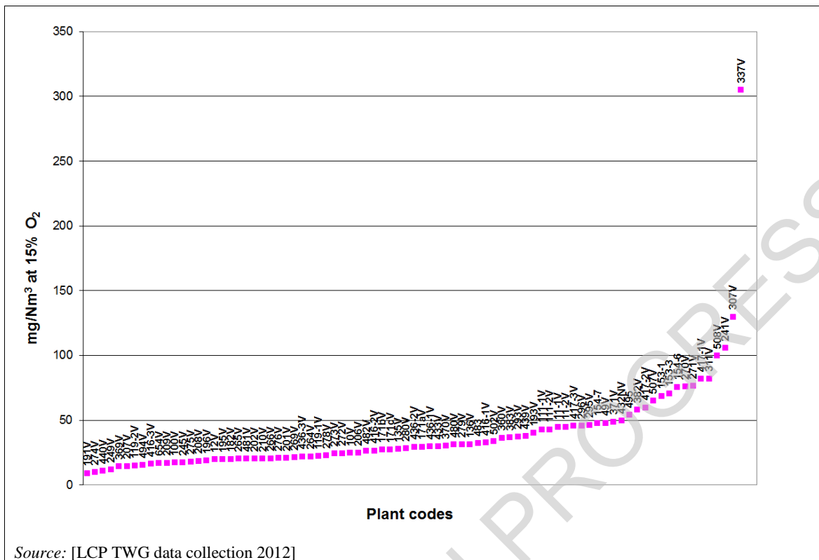
Figure 7.15: NO x emissions (yearly averages) from CCGTs without supplementary firing at the HRSG level
