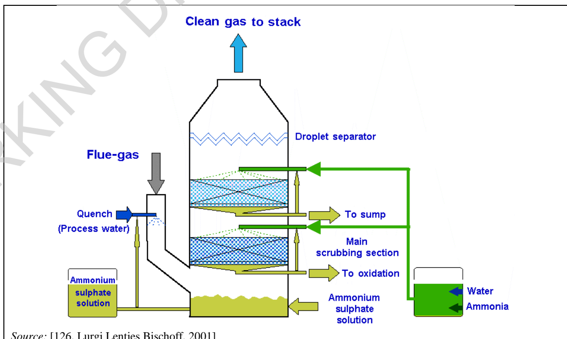
Figure 3.23: The ammonia wet scrubber
