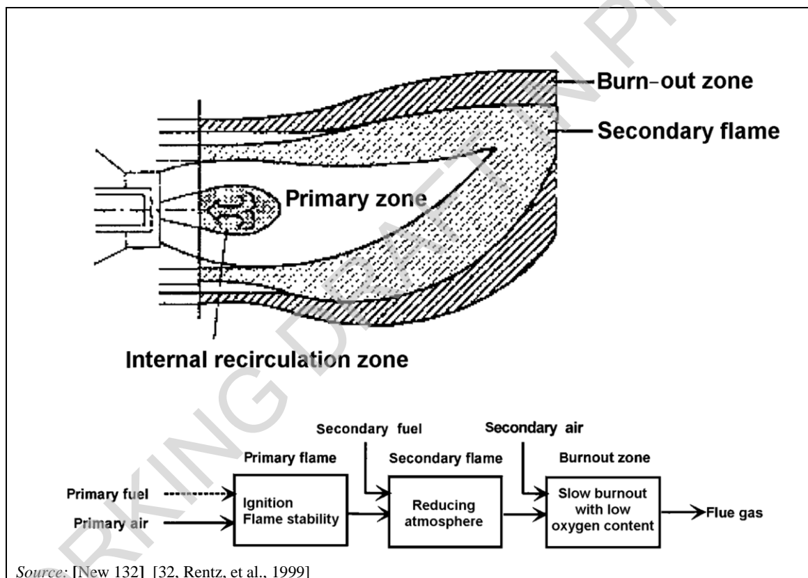
Figure 3.35: Fuel staging at the burner
