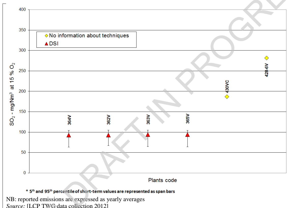
Figure 6.12: SO 2 emissions from well-performing HFO- and/or gas-oil-fired engines
