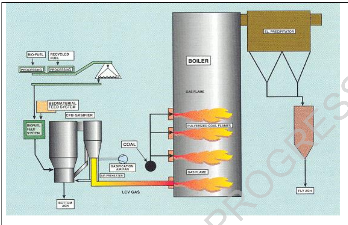
Figure 4.15: Kymijärvi CFB gasifier
