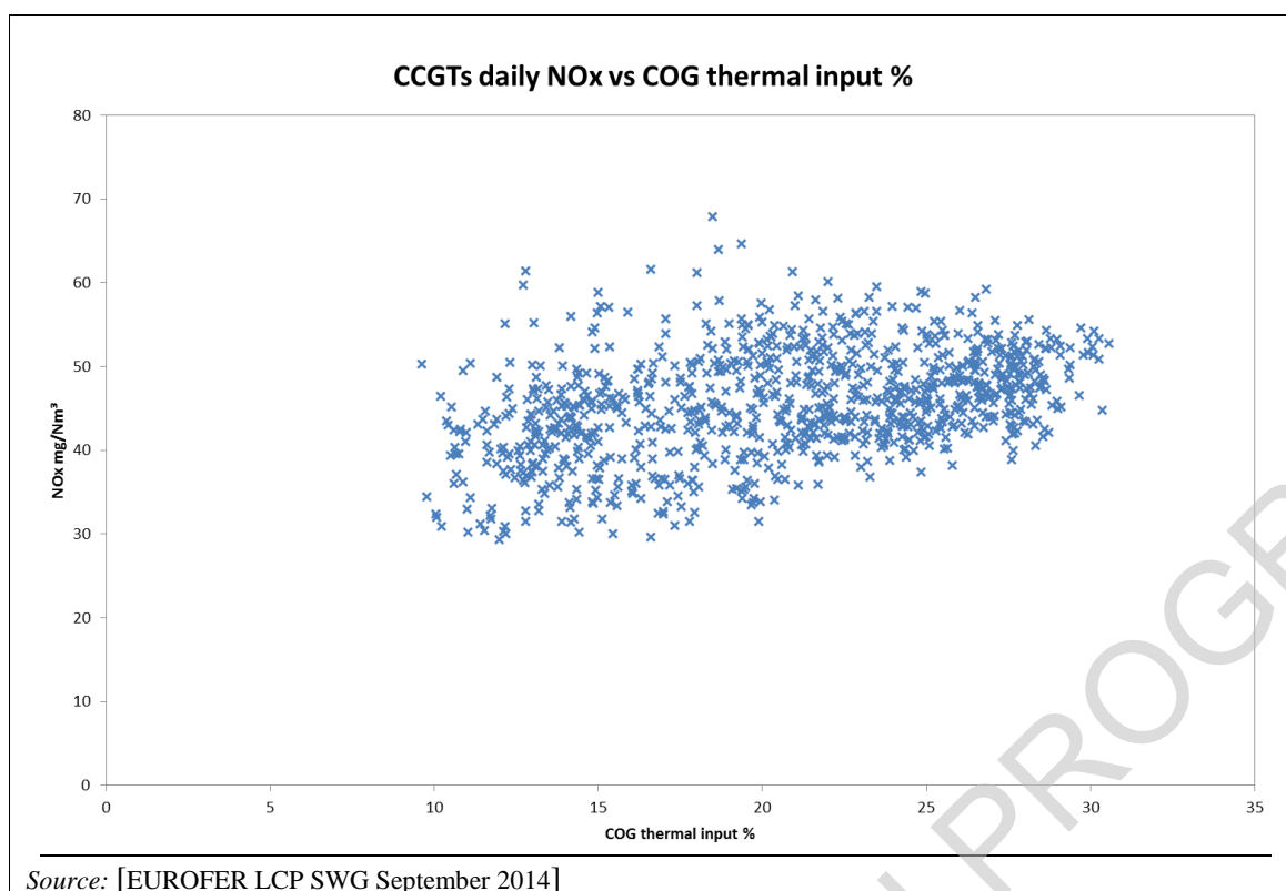
Figure 7.46: NO x emissions and relative thermal input for a combination of three CCGTs combusting COG, using daily average data for 2010
