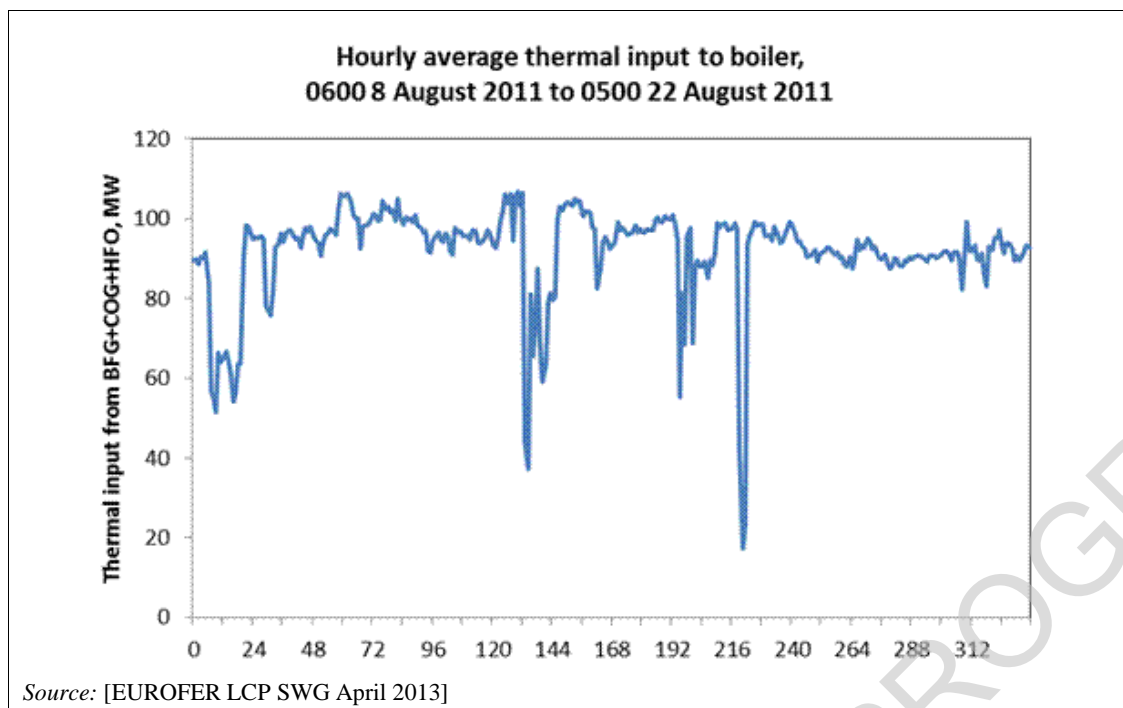
Figure 7.36: Hourly average thermal inputs of BF gas, COG and HFO to a boiler over a two-week period
