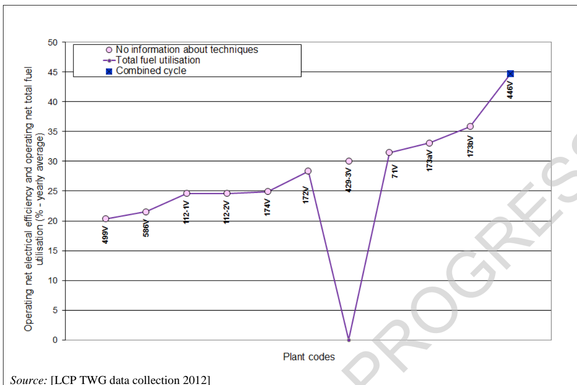
Figure 6.15: Operating energy efficiencies of European gas-oil-fired gas turbines
