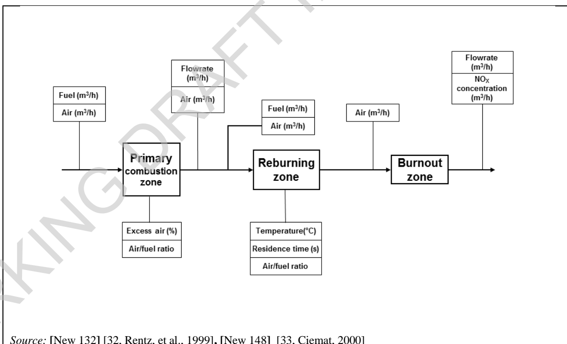
Figure 3.36: The three combustion zones and relevant parameters in a reburning process
