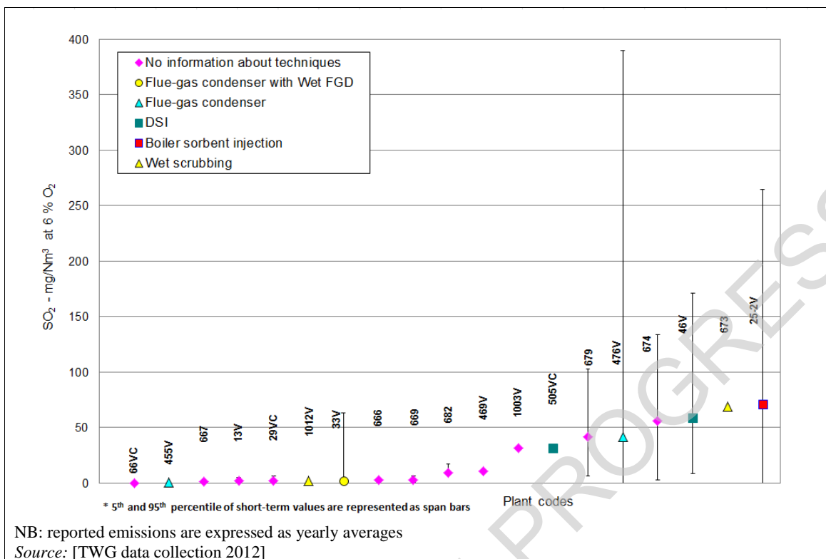
Figure 5.49: SO 2 emissions from well-performing biomass- and/or peat-fired plants between \geq 100 MW th and < 300 MW th
