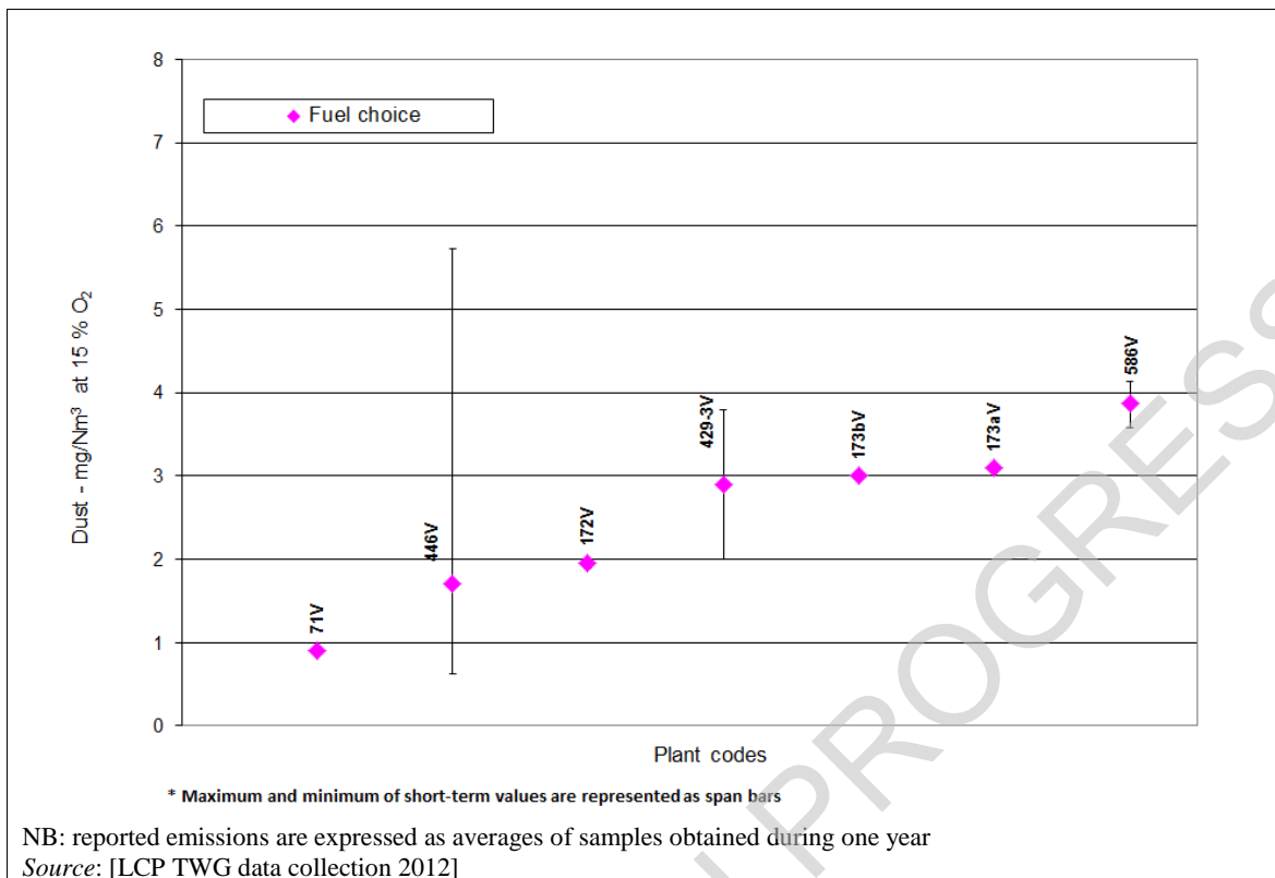
Figure 6.17: Dust emissions from well-performing gas-oil-fired gas turbines
