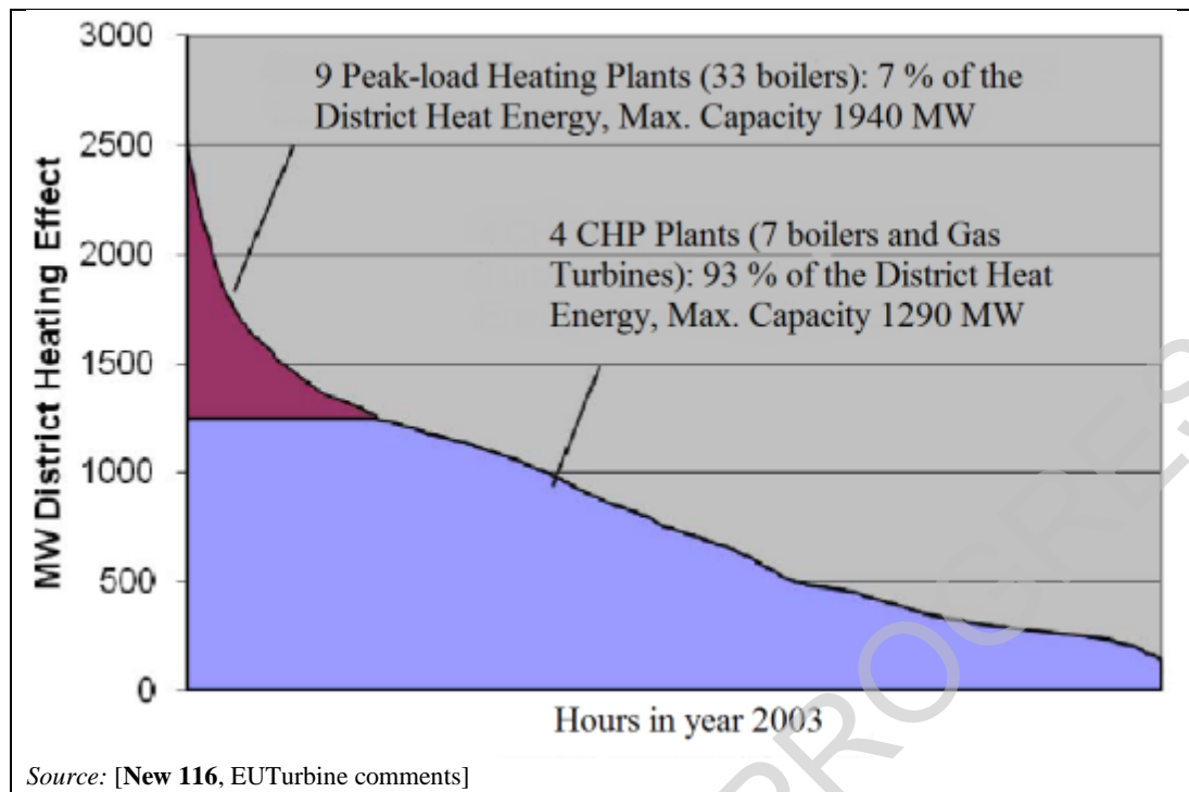
Figure 2.22: Duration curve of the district heating operation in the Helsinki region in 2003
