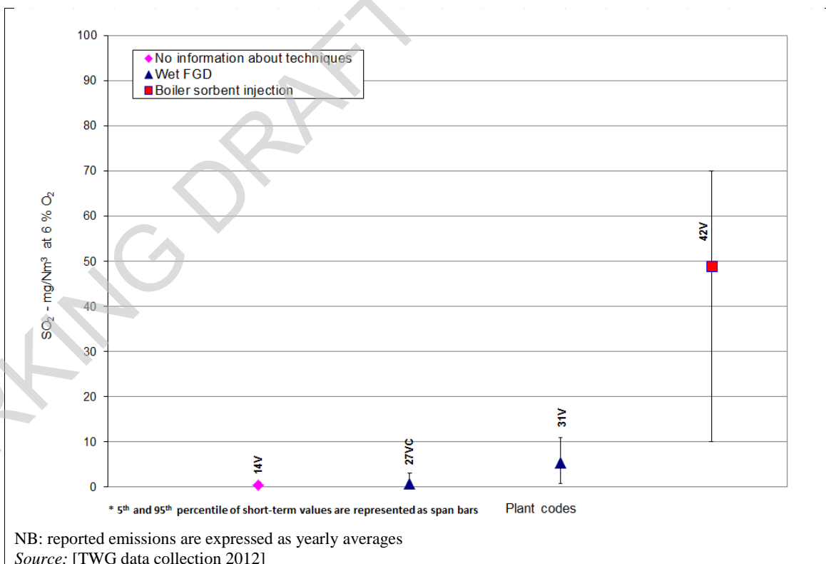
Figure 5.50: SO 2 emissions from well-performing biomass- and/or peat-fired plants of \geq 300 MW th
