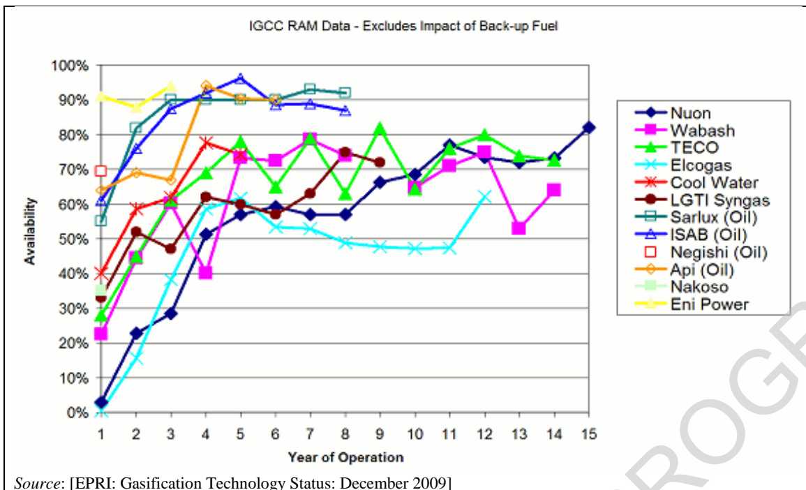
Figure 4.14: Availability statistics for IGCC first-of-a-kind plants
