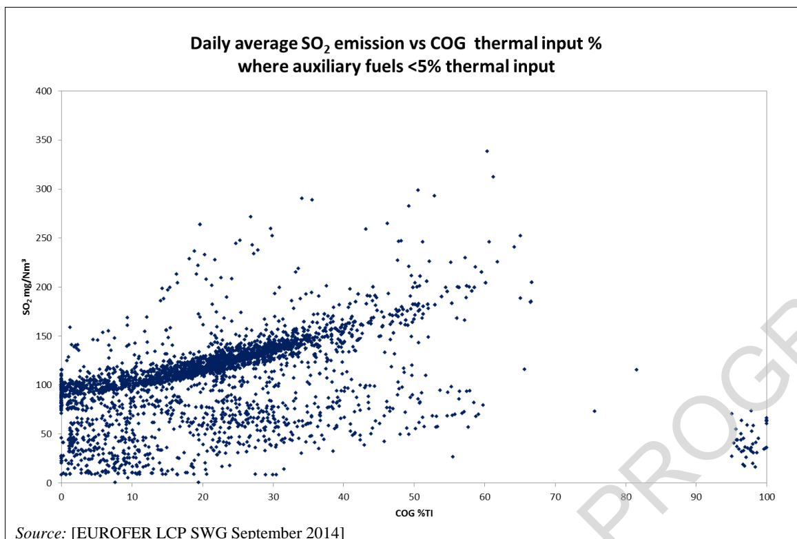
Figure 7.55: Relationship between the daily average SO 2 emission and COG thermal input (%) for boilers using iron and steel process gases (thermal input from auxiliary fuels < 5 %)
