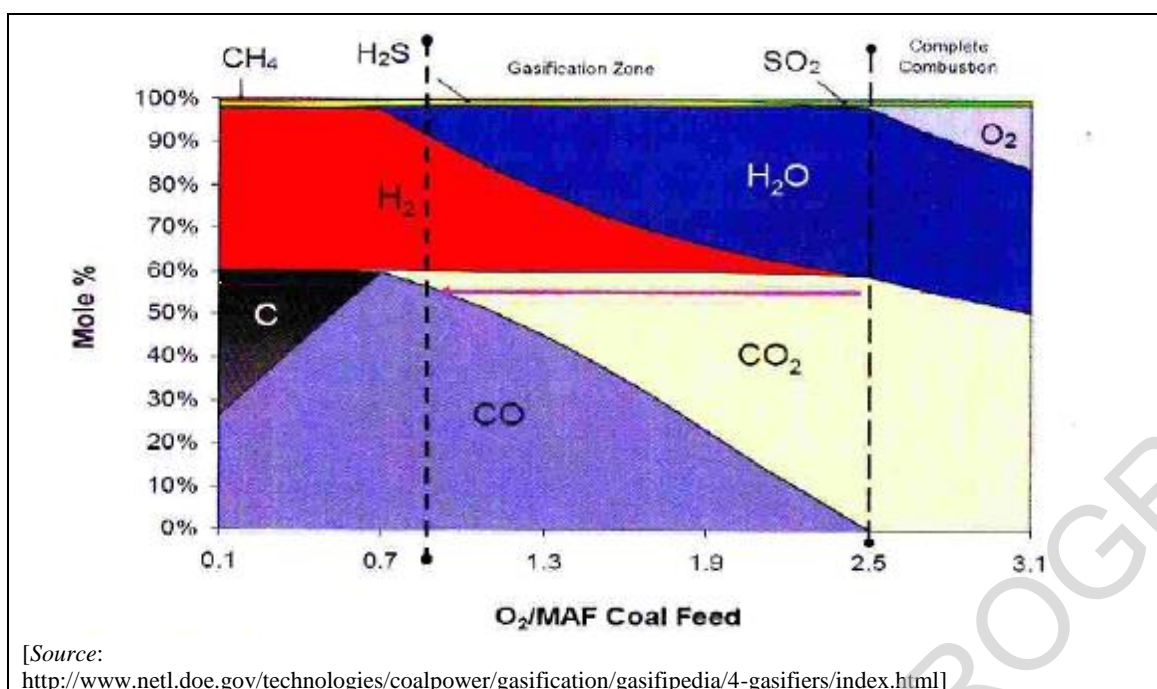
Figure 4.3: Syngas composition as a function of the O 2 to coal feed ratio
