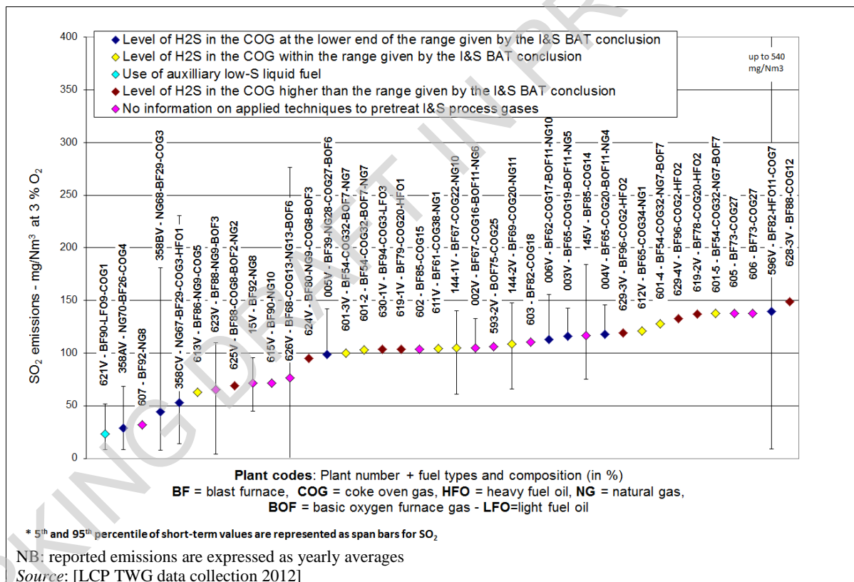
Figure 7.54: SO 2 emissions from well-performing boilers combusting iron and steel process gases
