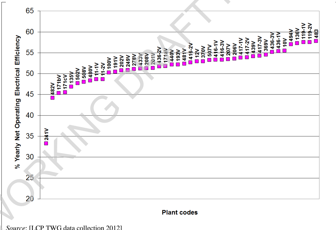
Figure 7.7: Net operating electrical efficiencies of CCGTs without supplementary firing in 2010
