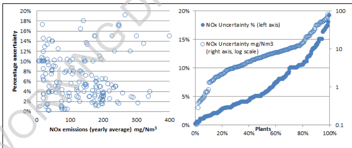
Figure 13.1: Measurement uncertainties reported for \text{NO}_x emissions
