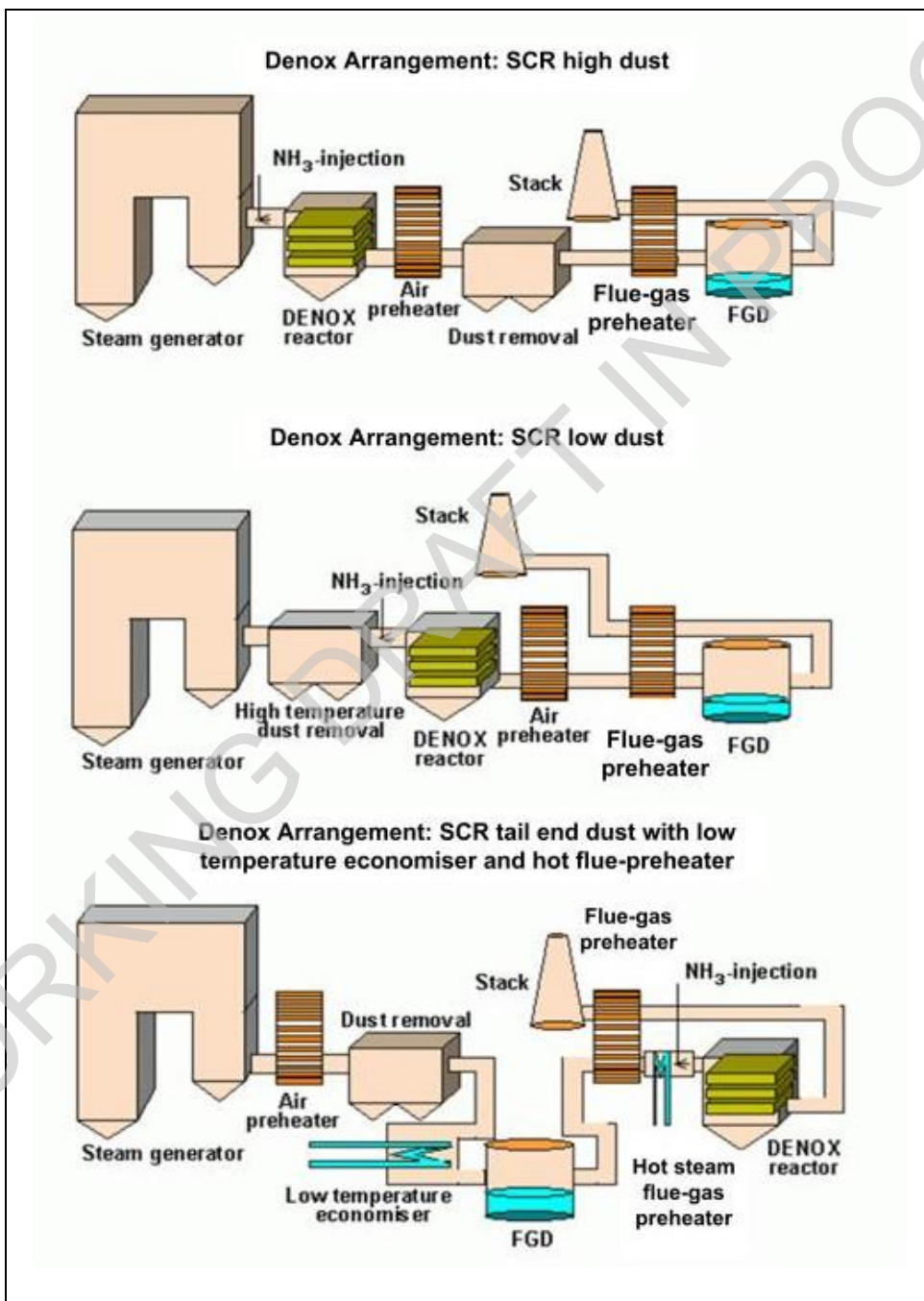
Figure 3.43: Existing configurations of SCR NO x abatement techniques
