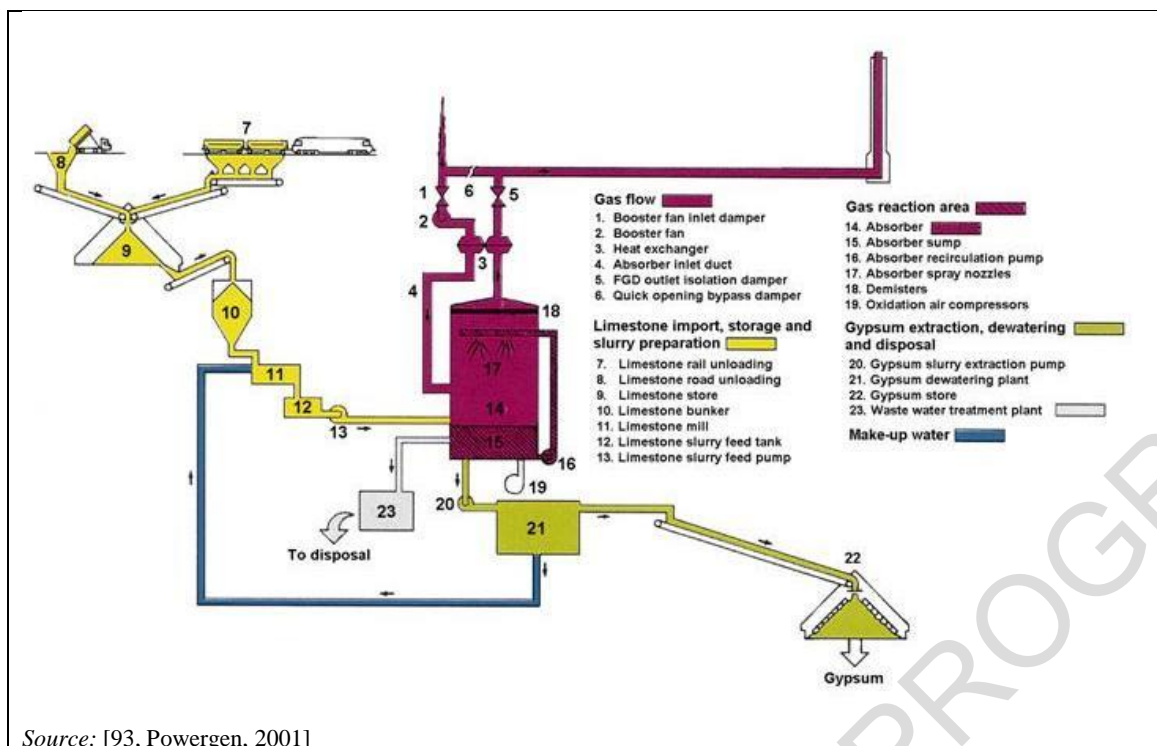
Figure 5.7: Wet FGD process with a spray tower
