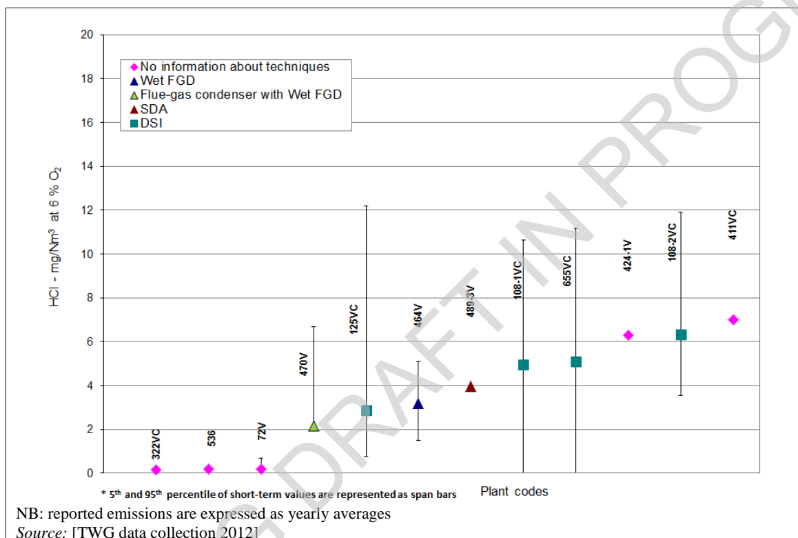
Figure 5.51: HCl emissions from well-performing biomass- and/or peat-fired plants of < 100 MW th
