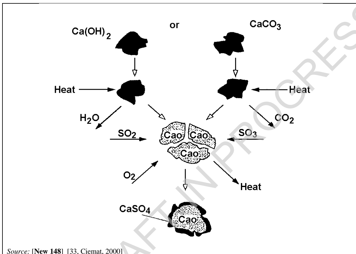
Figure 3.29: SO 2 removal reactions in furnace sorbent injection
