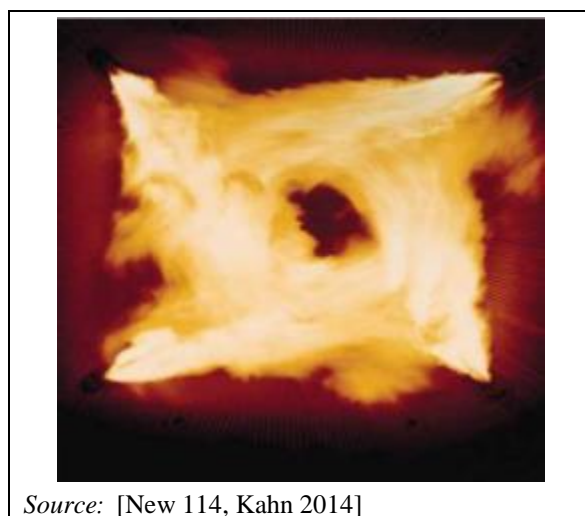
Figure 2.2: Tangential-fired combustion chamber
