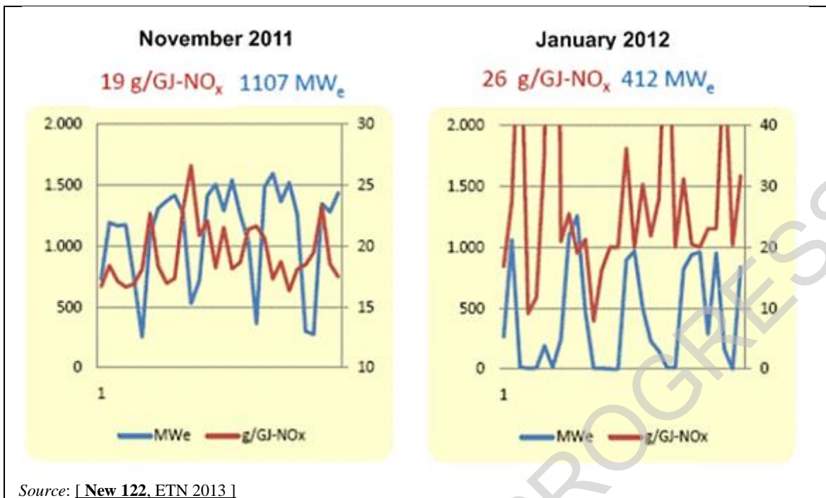
Figure 3.10: Impact of load factor variation on NO x emissions at a GDF Suez natural gas combined-cycle plant, including five units of 385 MW e
