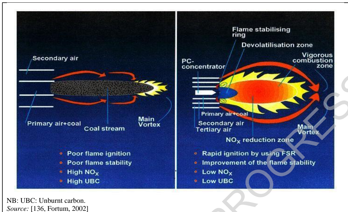
Figure 3.33: Comparison of conventional air-staged and advanced air-staged low- \text{NO}_x burners
