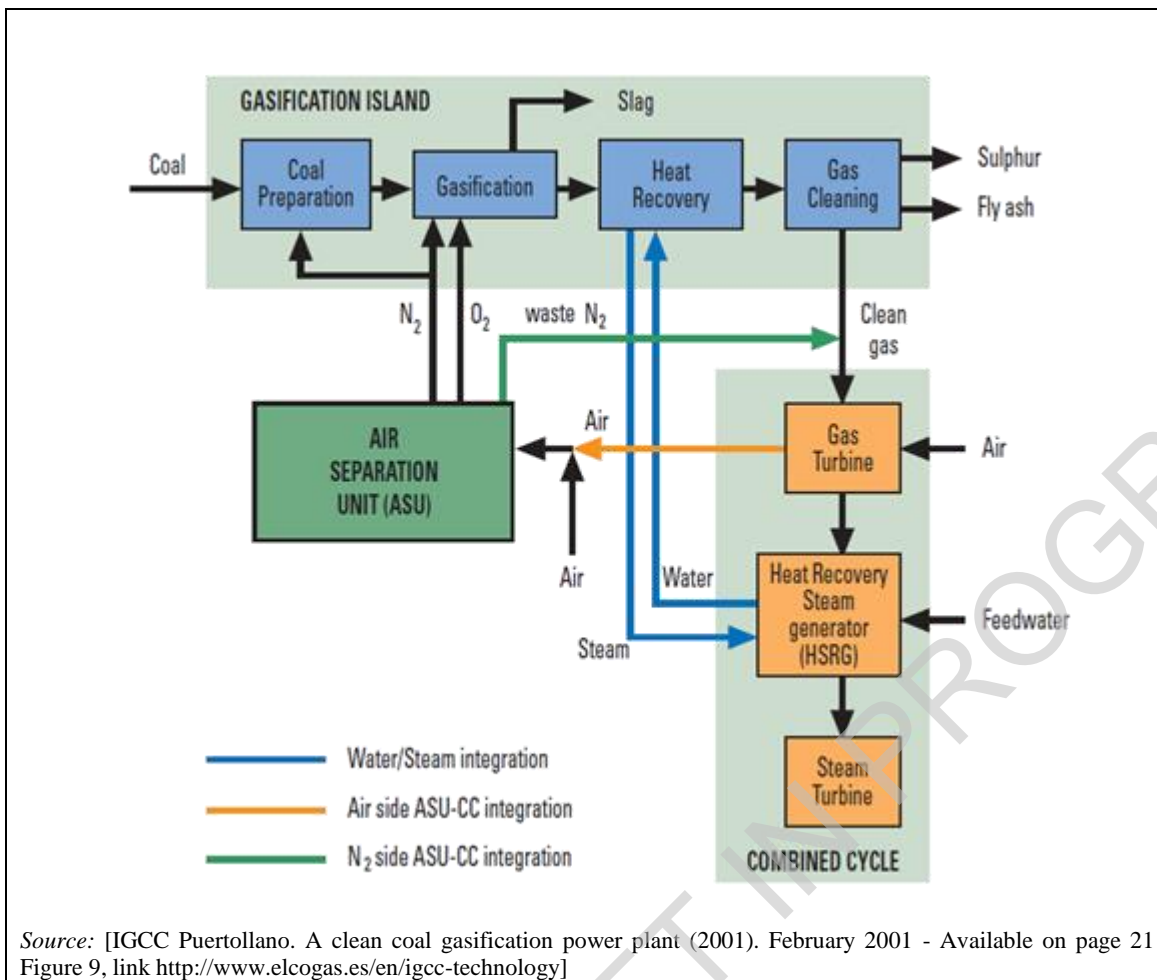
Figure 4.1: Block diagram and integration options for an IGCC plant
