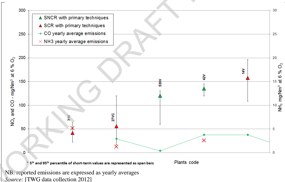
Figure 5.47: NO x s from well-performing biomass- and/or peat-fired plants of ≥ 300 MW th
