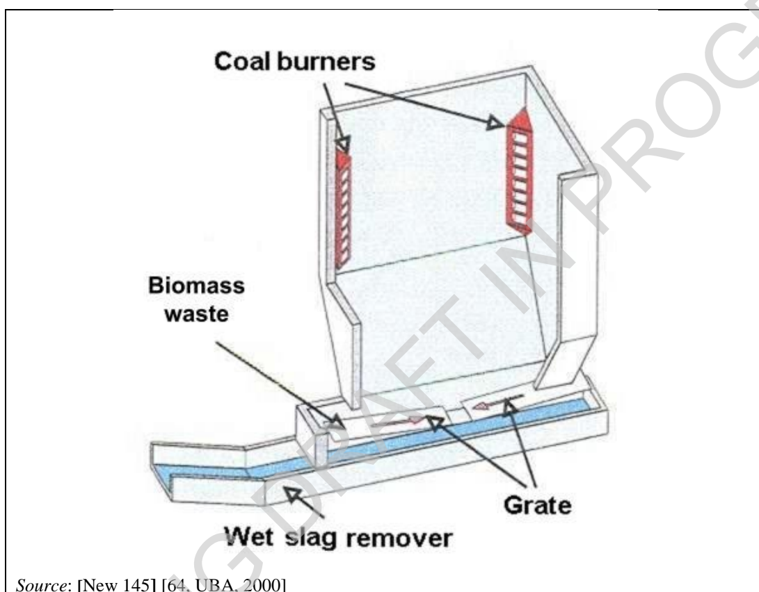
Figure 9.2: Internal grates in a pulverised coal-fired boiler
