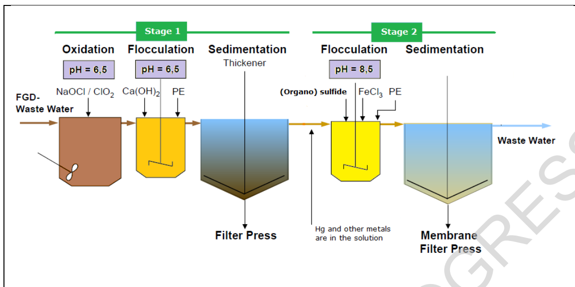
Figure 3.7: Two-stage waste water treatment plant
