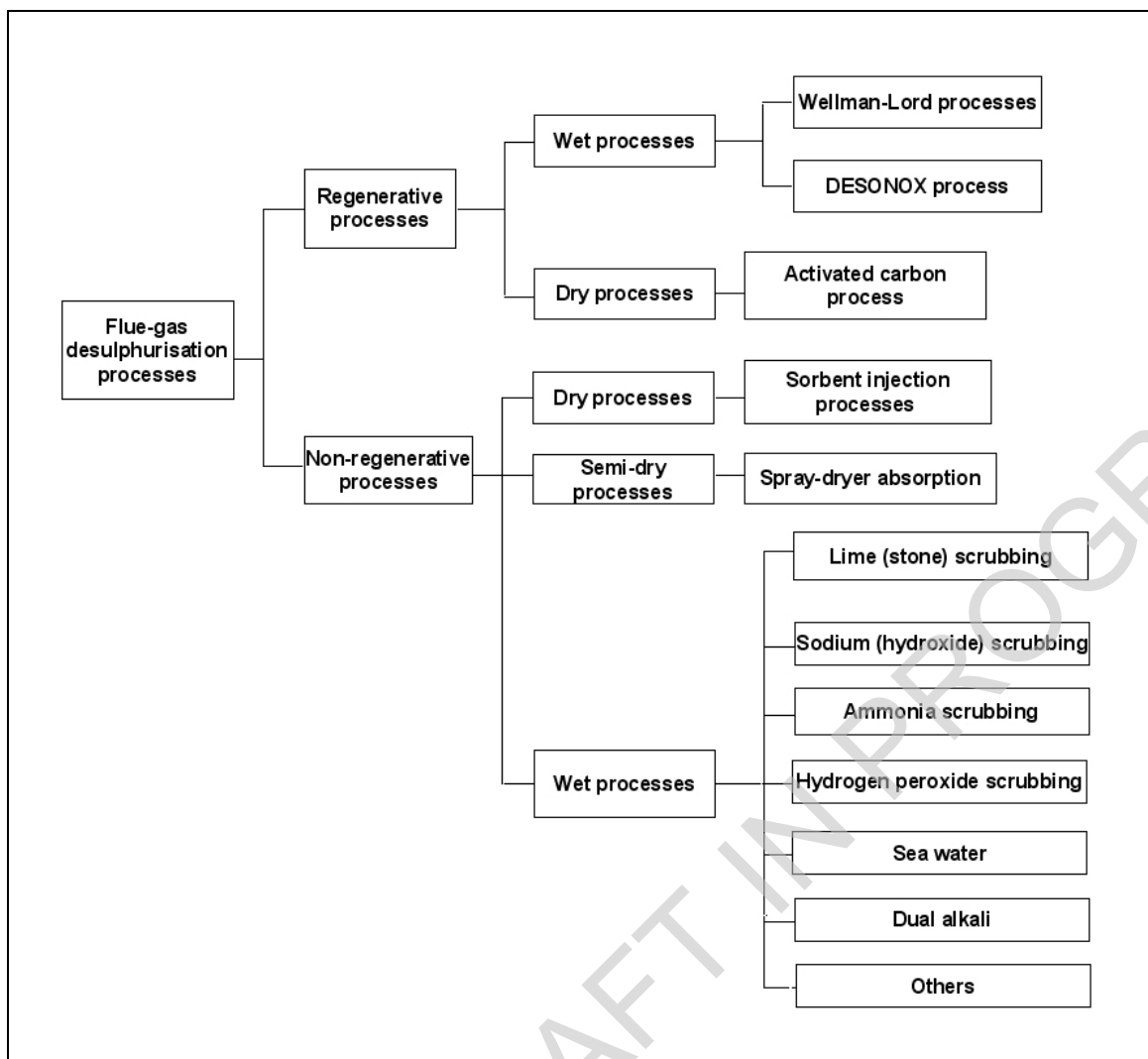
Figure 3.2: Overview of secondary techniques used to reduce sulphur oxide emissions
