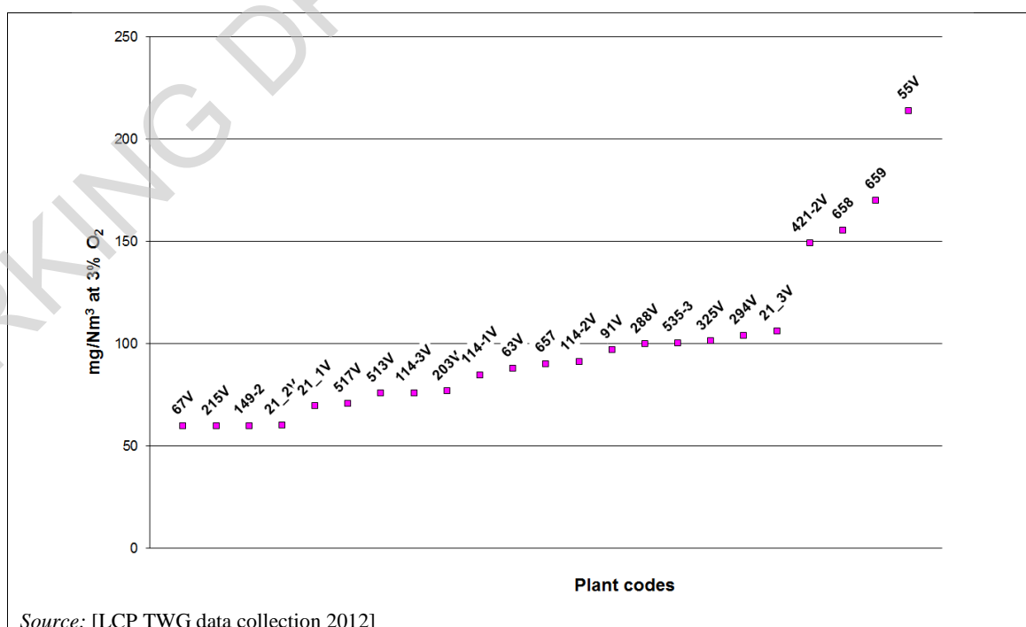
Figure 7.16: NO x emissions (yearly averages) from European natural gas boilers in 2010
