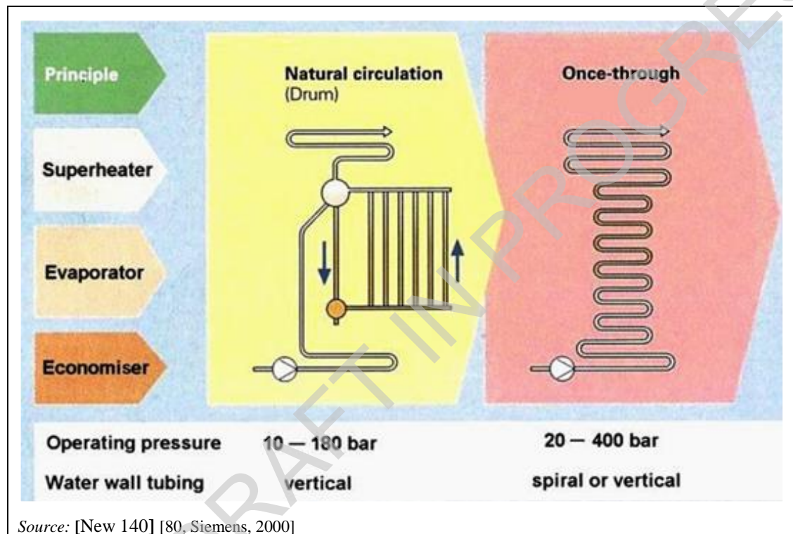
Figure 2.19: The natural circulation and once-through boiler concepts
