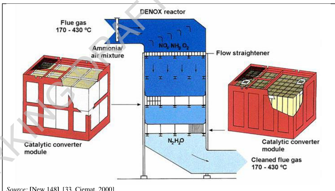
Figure 3.42: Configuration of catalyst reactor
