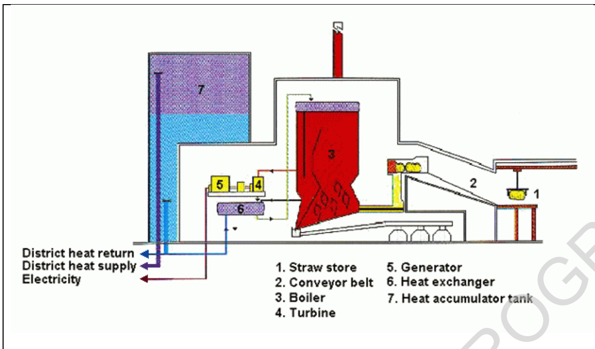
Figure 5.40: Straw-firing combustion plant
