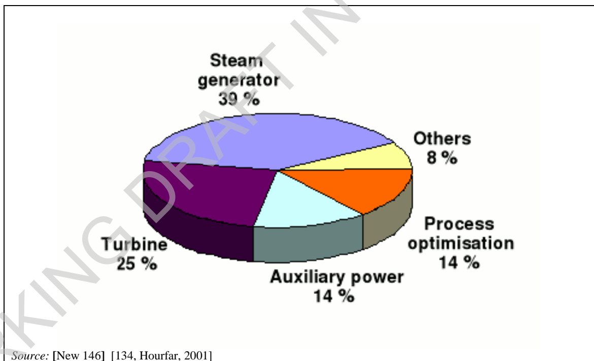
Figure 2.28: Improvements in the efficiency of power plants between 1993 and 2000
