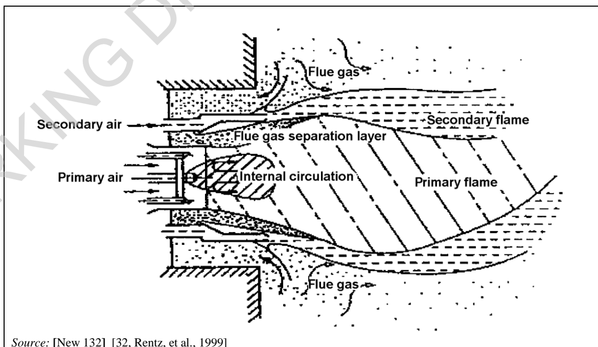
Figure 3.34: Flue-gas recirculation low- \text{NO}_x burners
