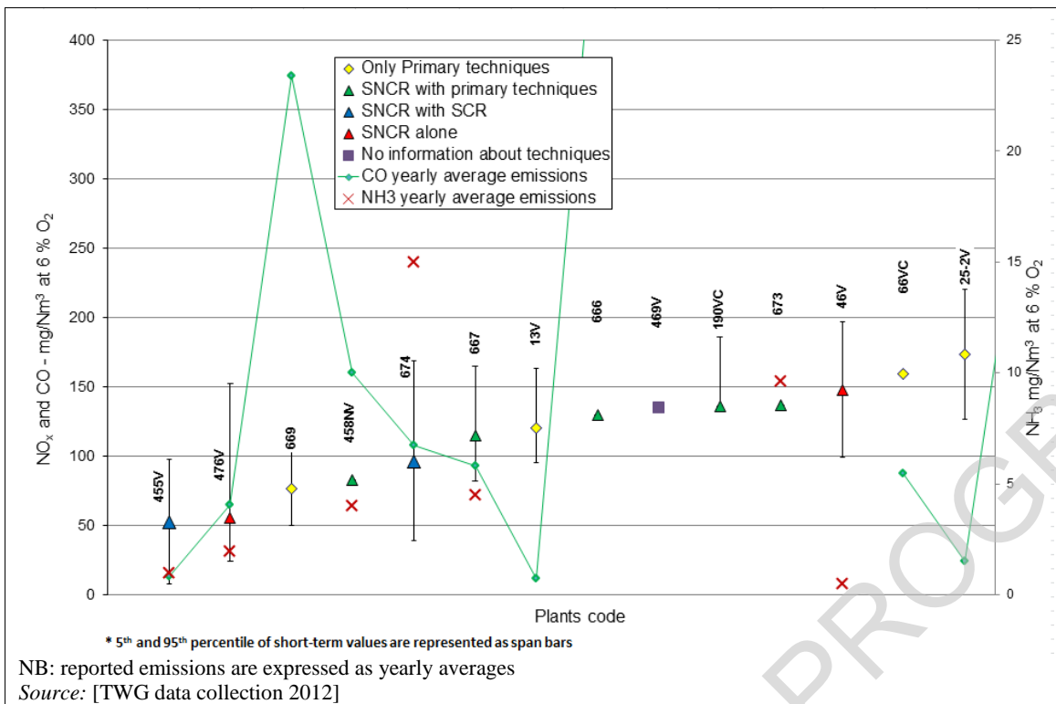
Figure 5.46: NO x s from well-performing biomass- and/or peat-fired plants between 100 MW th and 300 MW th
