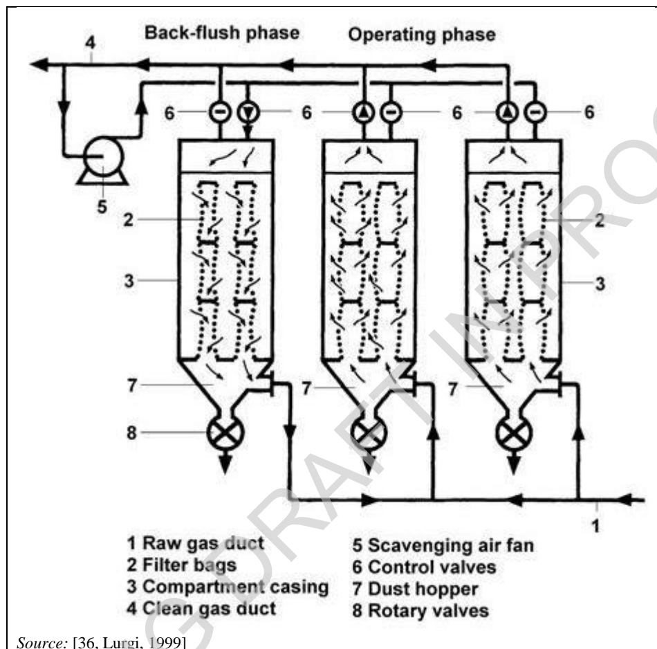
Figure 3.14: General arrangement of a bag filter (with one compartment in the cleaning cycle)
