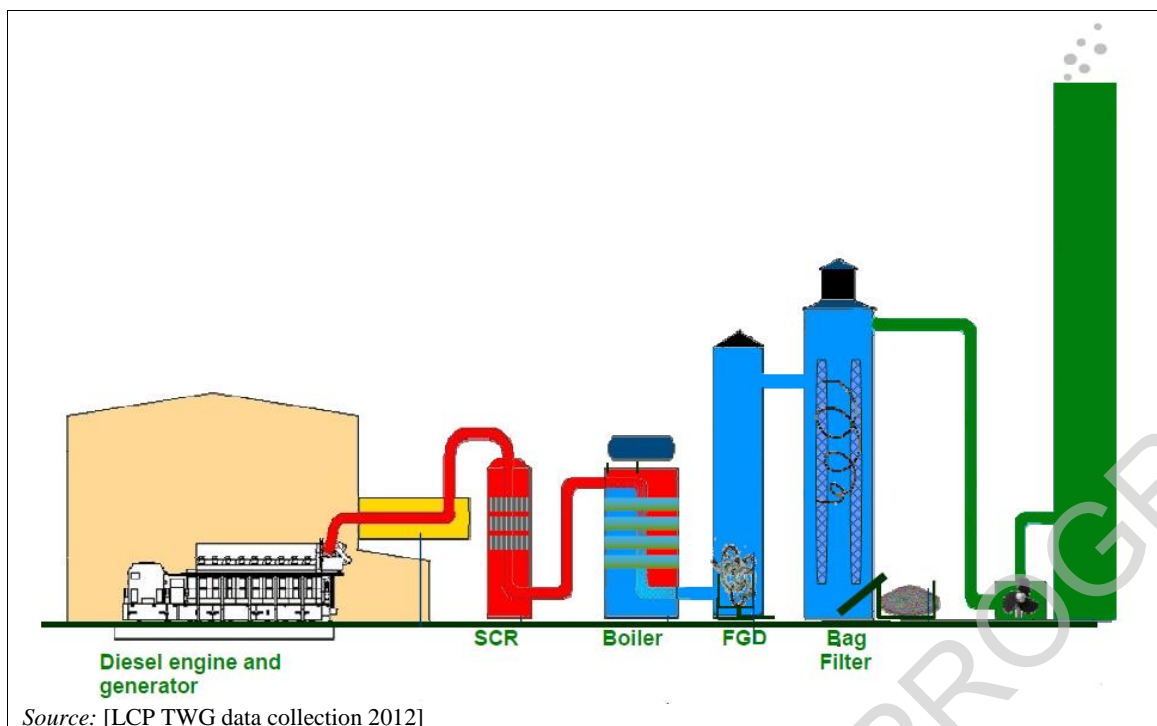
Figure 6.14: Configuration of an engine combustion plant fitted with SCR, recovery boiler, DSI and a bag filter
