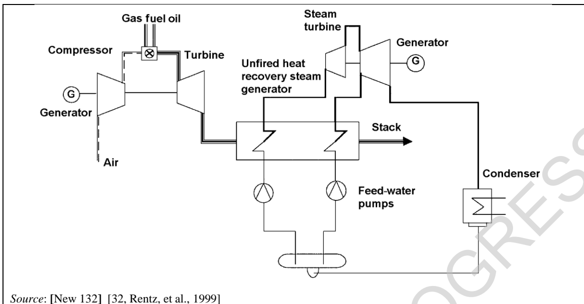
Figure 3.56: Schematic of a combined-cycle power plant with a heat recovery steam generator (HRSG)
