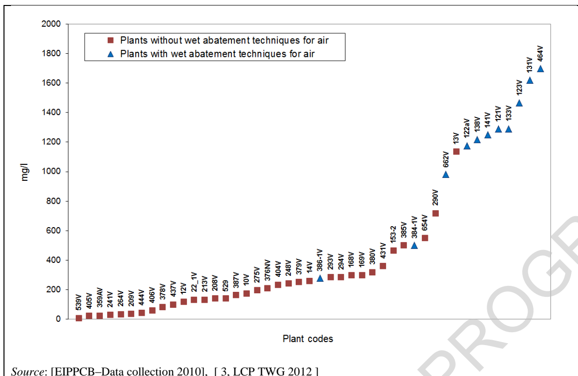
Figure 3.8: Yearly sulphate concentration in the direct emission of the plants – Comparison of plants with a wet abatement system for air pollutants and plants without
