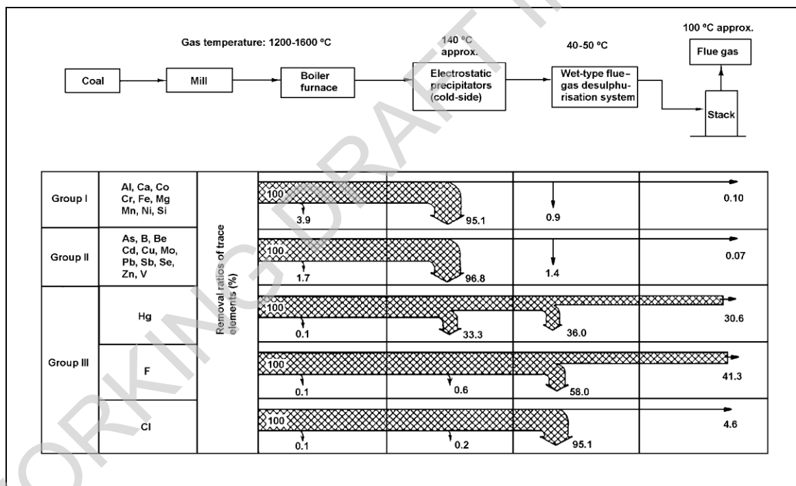
Figure 3.5: Mass balance of metals, fluoride and chloride in coal-fired combustion plants
