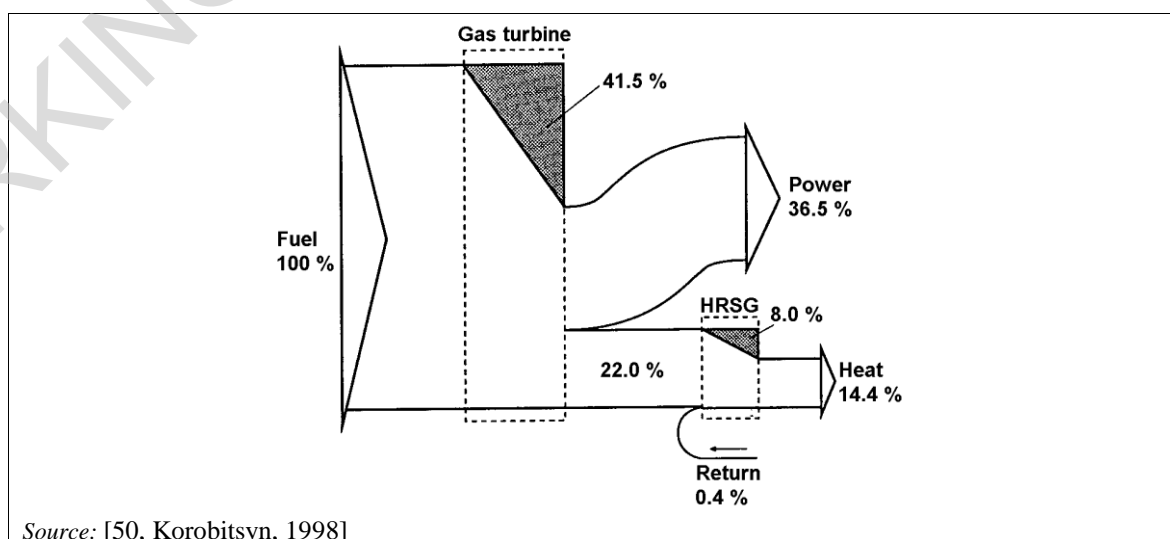
Figure 7.4: Grassmann diagram of a gas turbine with HRSG
