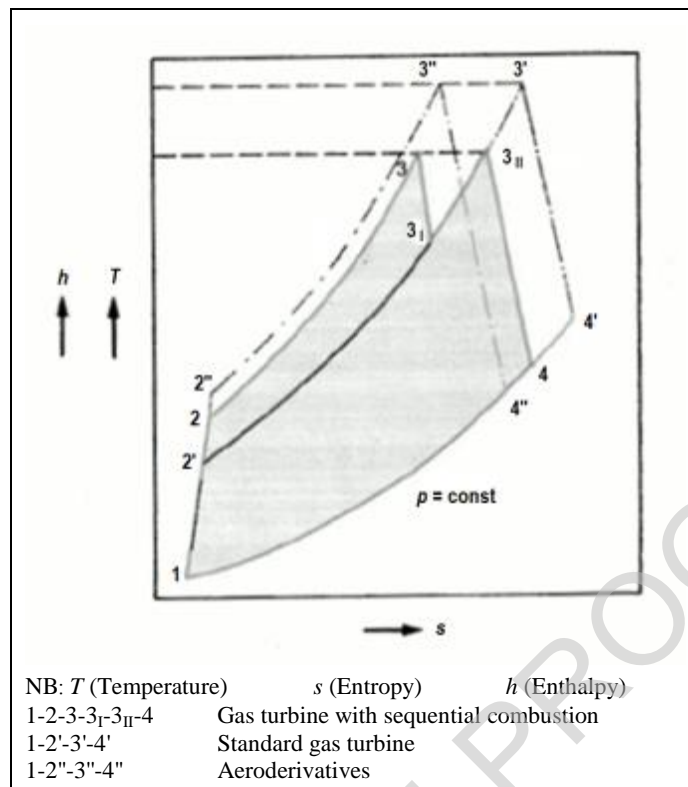
Figure 2.13: Scheme of a gas turbine process with sequential combustion
