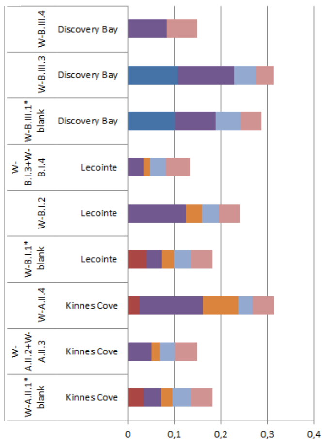
Figure 2: levels of PFASs found in water samples
