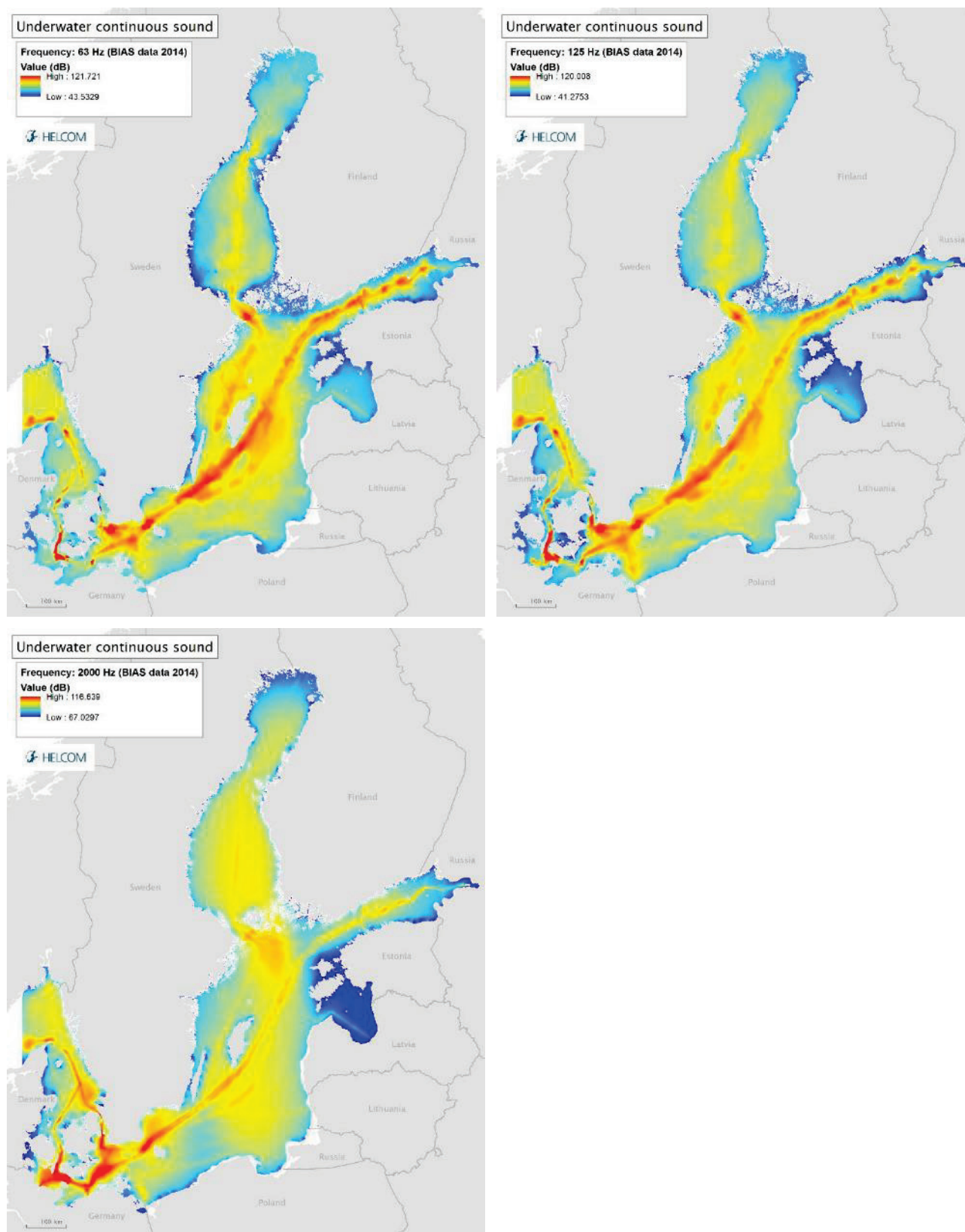
Figure 4.4.1. Soundscape maps in the Baltic Sea , showing underwater continuous sound at 1/3 octave frequency bands of 63 Hz, 125 Hz and 2000 Hz. Areas with high sound level overlap clearly with the location of major shipping routes. The sound produced from shipping is within a frequency interval that overlaps with the hearing range of several species. The results have been extracted with help of the soundscape planning tool of BIAS (2016).
