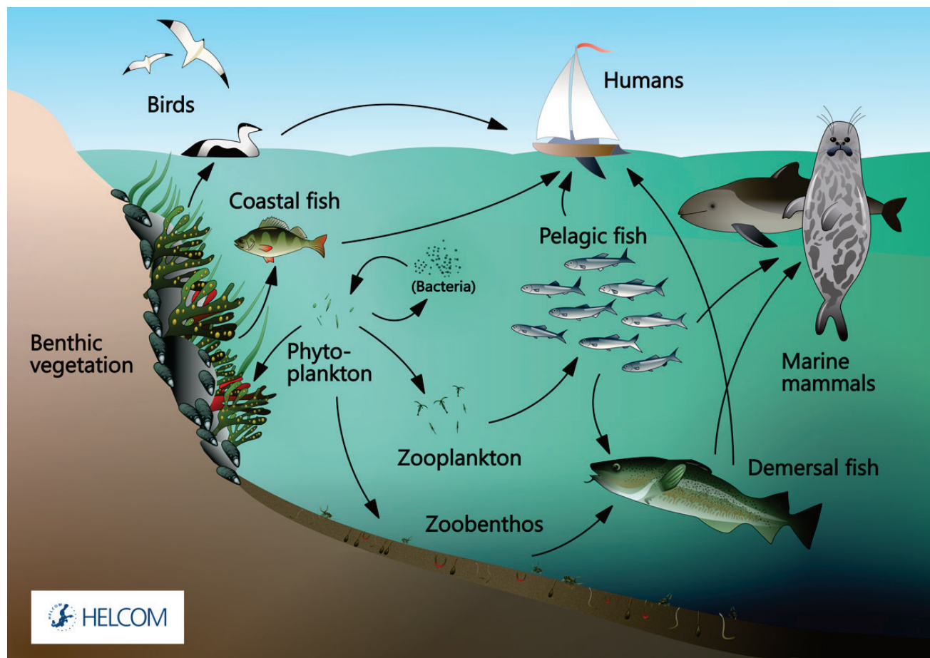
Figure 1.3. A schematic, simplified illustration of the food web structure in the Baltic Sea.
