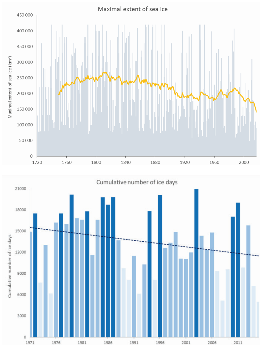
Figure 1.4. Changes over time in the maximum extent of sea ice during winter (km 2 ) since 1720, and in the cumulative number of ice days per winter since 1971. Yellow line shows the 30-year moving average. The extent of sea ice has clearly declined in past decades and the cumulative number of ice days show a decreasing trend. Source: Finnish Meteorological Institute.
