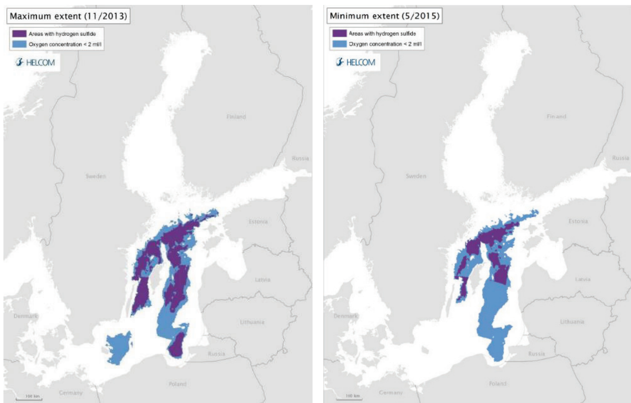
Figure 1.9. Poor oxygen conditions at the sea floor restrict productivity and biodiversity in the Baltic Sea. The maps show the minimum and maximum distribution of anoxic areas in the deep-water (where hydrogen sulphide is present) and areas with less than 2 ml/l oxygen during 2011–2015, based on point measurements and modelling. Data from Leibniz Institute for Baltic Sea Research Warnemuende. See also Feistel et al. (2016). Due to the range of input data used, the map may not correctly reflect the situation in the Gulf of Finland.
