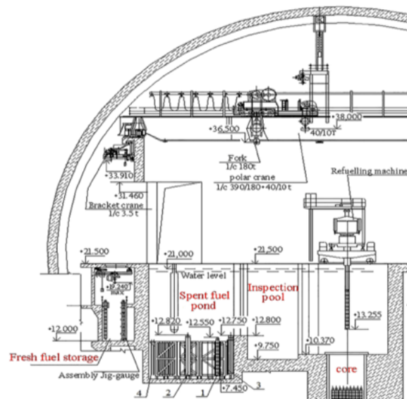
VVER-1000/320 reactor containment showing location of spent fuel pool 37
