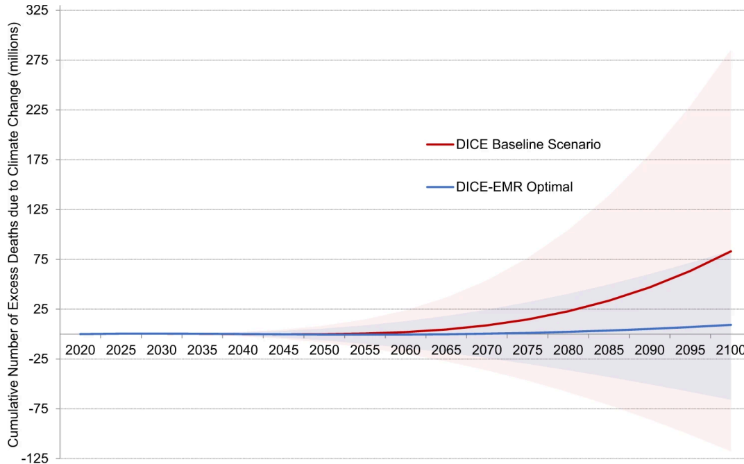
Figure 1. Cumulative excess deaths by 2100 in the central estimate of the DICE model's baseline emission scenario (Red). The red shaded region shows the range between the high (>90th percentile) and low (<10th percentile) projections for excess deaths. The blue line and shaded region shows the central estimate and range between high and low projections for excess deaths in the DICE-EMR optimal emissions path as used in the Greenpeace Netherlands report (Source: Bressler, 2021 6 ).
