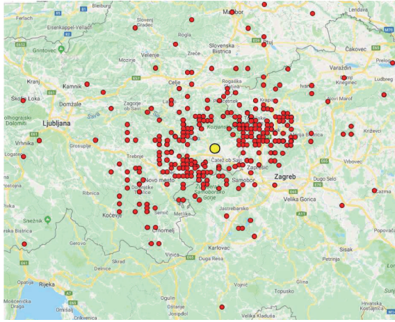
Figure 2: Maximum distances for necessary evacuation after a severe accident at the Krško NPP (JOE 2019)
