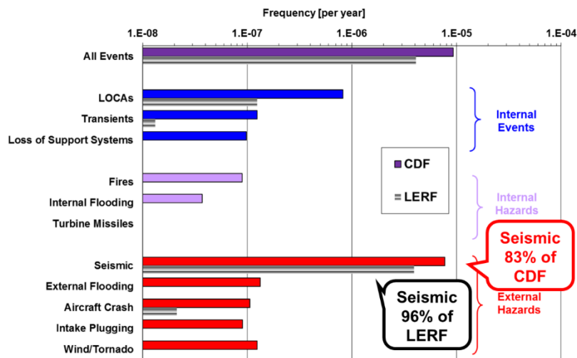
Figure 3: Core damage frequency (CDF) und Large early releases frequency (LERF) at Beznau NPP (Status 2015) (RICHTER 2015)
