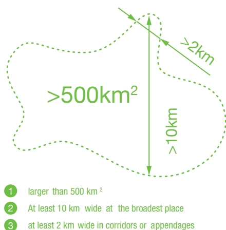
Figure 3 : Geometrical rules defining an IFL area (Potapov, 2008)
