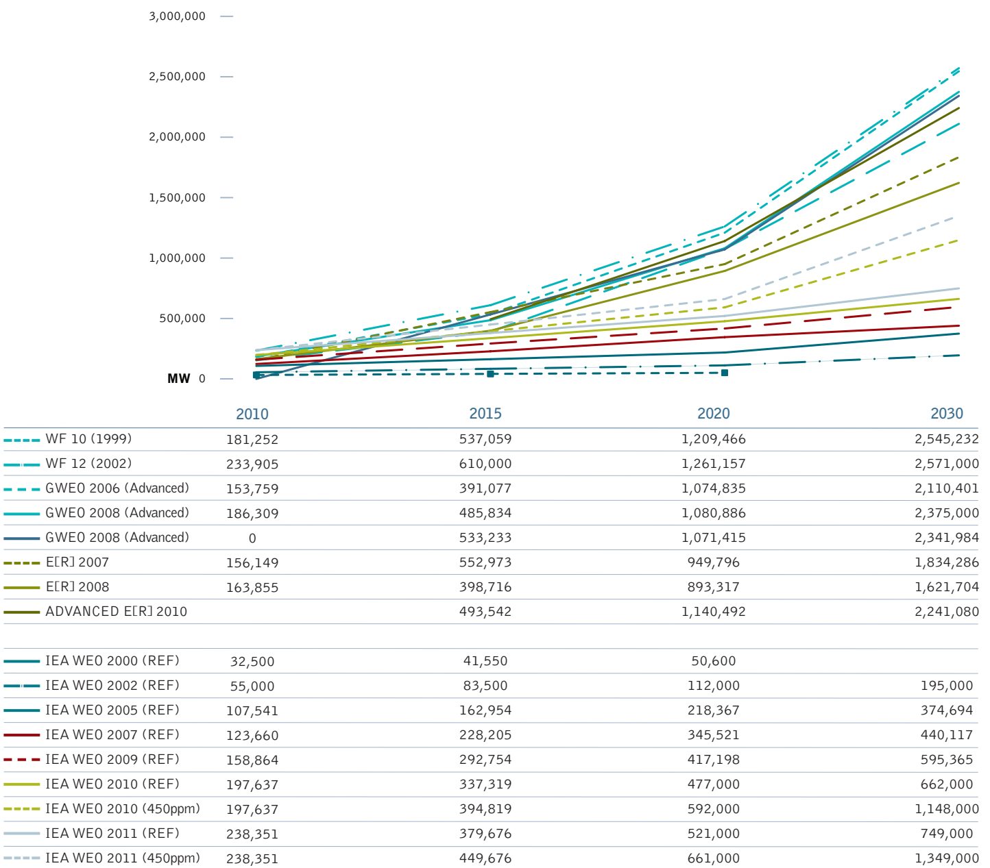
figure 4.6: wind power: long term market projections until 2030
