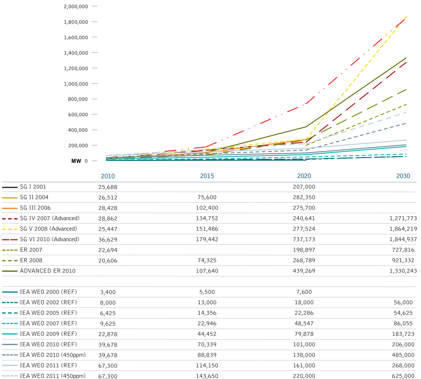
figure 4.8: photovoltaic: long term market projections until 2030
