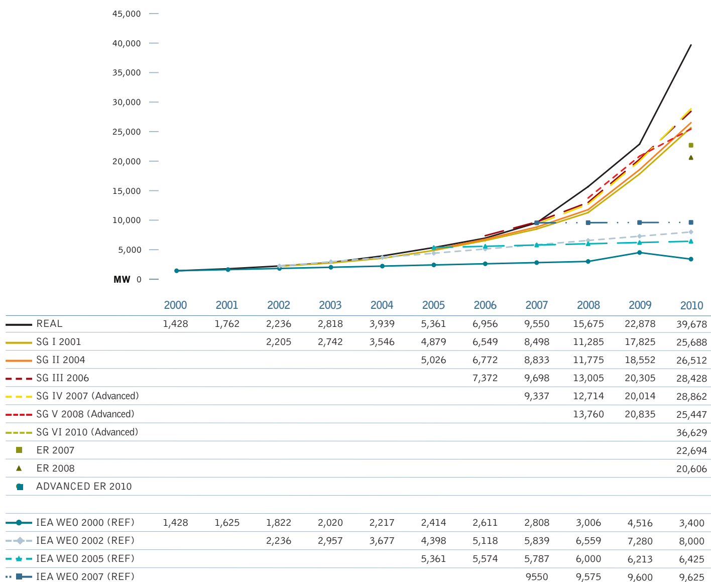
figure 4.7: photovoltaics: short term prognosis vs real market development - global cumulative capacity
