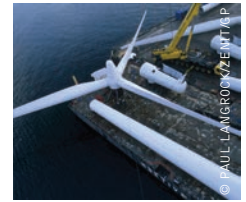
image CONSTRUCTION OF THE OFFSHORE WINDFARM AT MIDDELGRUNDEN NEAR COPENHAGEN, DENMARK.
